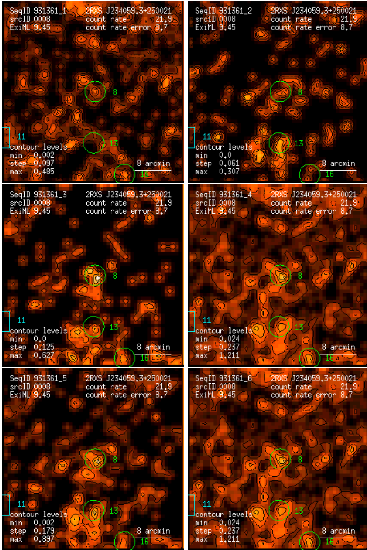
Figure 8: RASS 931361: detection 0008: band rate images, Gaussian filter: (1) PSPC channels 11 – 41, (2) 52 – 90, (3) 91 – 201, (4) 11 – 235, (5) 52 – 201, (6) 11 – 201. Broad band rates in counts/ks. Band rate contour levels in counts/ks/arcmin 2 .
