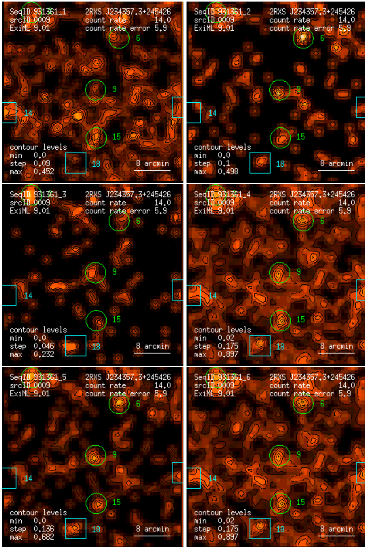
Figure 9: RASS 931361: detection 0009: band rate images, Gaussian filter: (1) PSPC channels 11 – 41, (2) 52 – 90, (3) 91 – 201, (4) 11 – 235, (5) 52 – 201, (6) 11 – 201. Broad band rates in counts/ks. Band rate contour levels in counts/ks/arcmin 2 .
