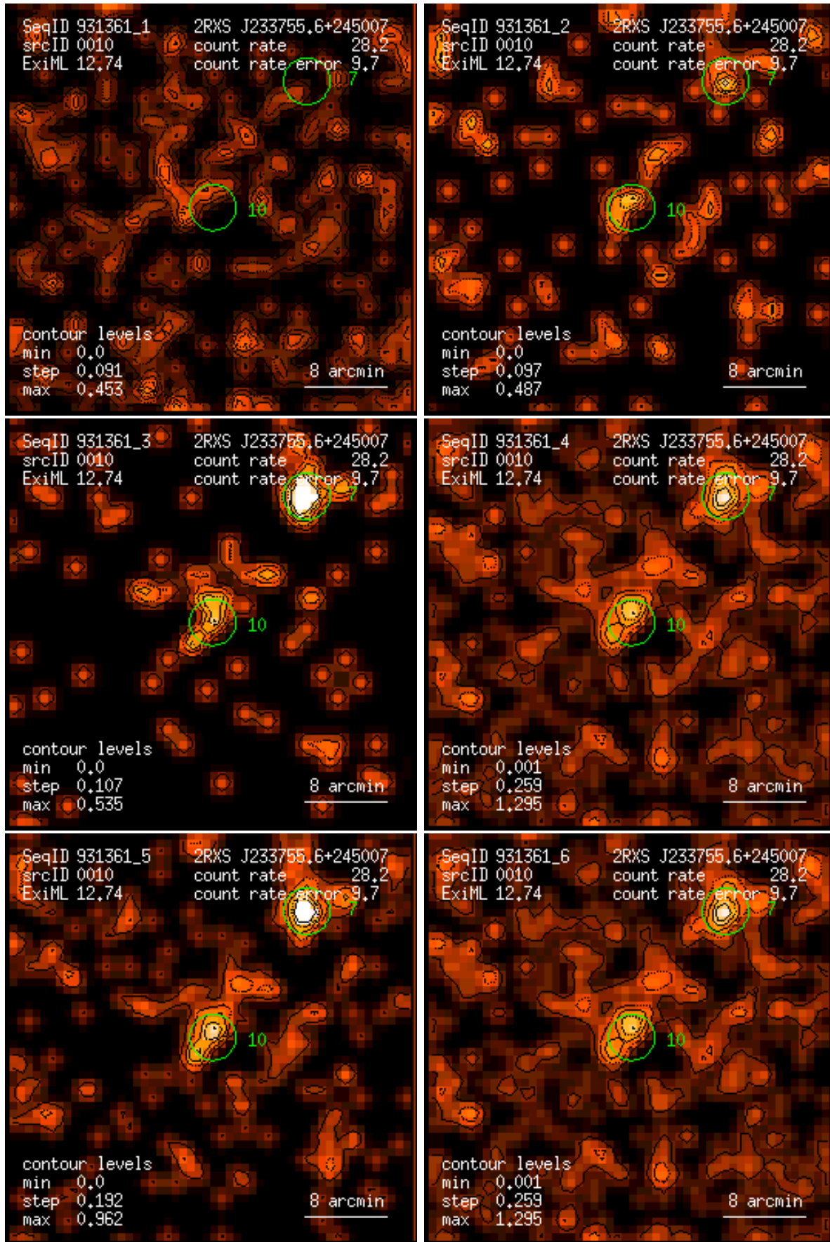
Figure 10: RASS 931361: detection 0010: band rate images, Gaussian filter: (1) PSPC channels 11 – 41, (2) 52 – 90, (3) 91 – 201, (4) 11 – 235, (5) 52 – 201, (6) 11 – 201. Broad band rates in counts/ks. Band rate contour levels in counts/ks/arcmin 2 .
