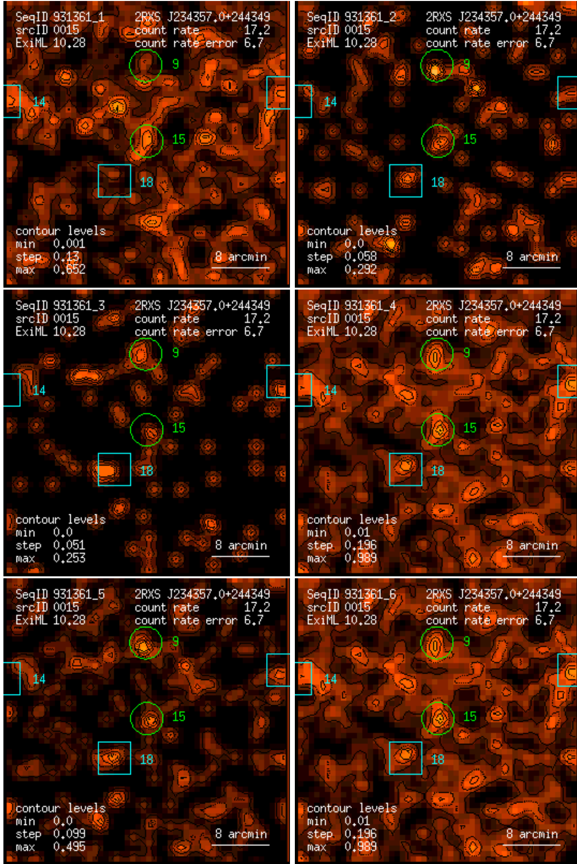
Figure 15: RASS 931361: detection 0015: band rate images, Gaussian filter: (1) PSPC channels 11 – 41, (2) 52 – 90, (3) 91 – 201, (4) 11 – 235, (5) 52 – 201, (6) 11 – 201. Broad band rates in counts/ks. Band rate contour levels in counts/ks/arcmin 2 .
