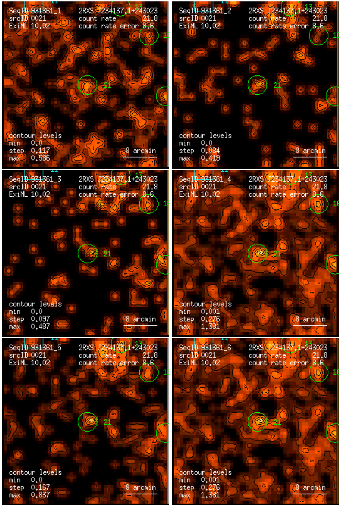
Figure 21: RASS 931361: detection 0021: band rate images, Gaussian filter: (1) PSPC channels 11 – 41, (2) 52 – 90, (3) 91 – 201, (4) 11 – 235, (5) 52 – 201, (6) 11 – 201. Broad band rates in counts/ks. Band rate contour levels in counts/ks/arcmin 2 .
