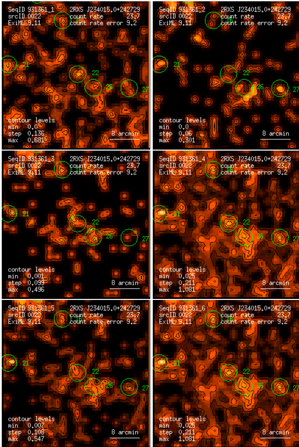
Figure 22: RASS 931361: detection 0022: band rate images, Gaussian filter: (1) PSPC channels 11 – 41, (2) 52 – 90, (3) 91 – 201, (4) 11 – 235, (5) 52 – 201, (6) 11 – 201. Broad band rates in counts/ks. Band rate contour levels in counts/ks/arcmin 2 .
