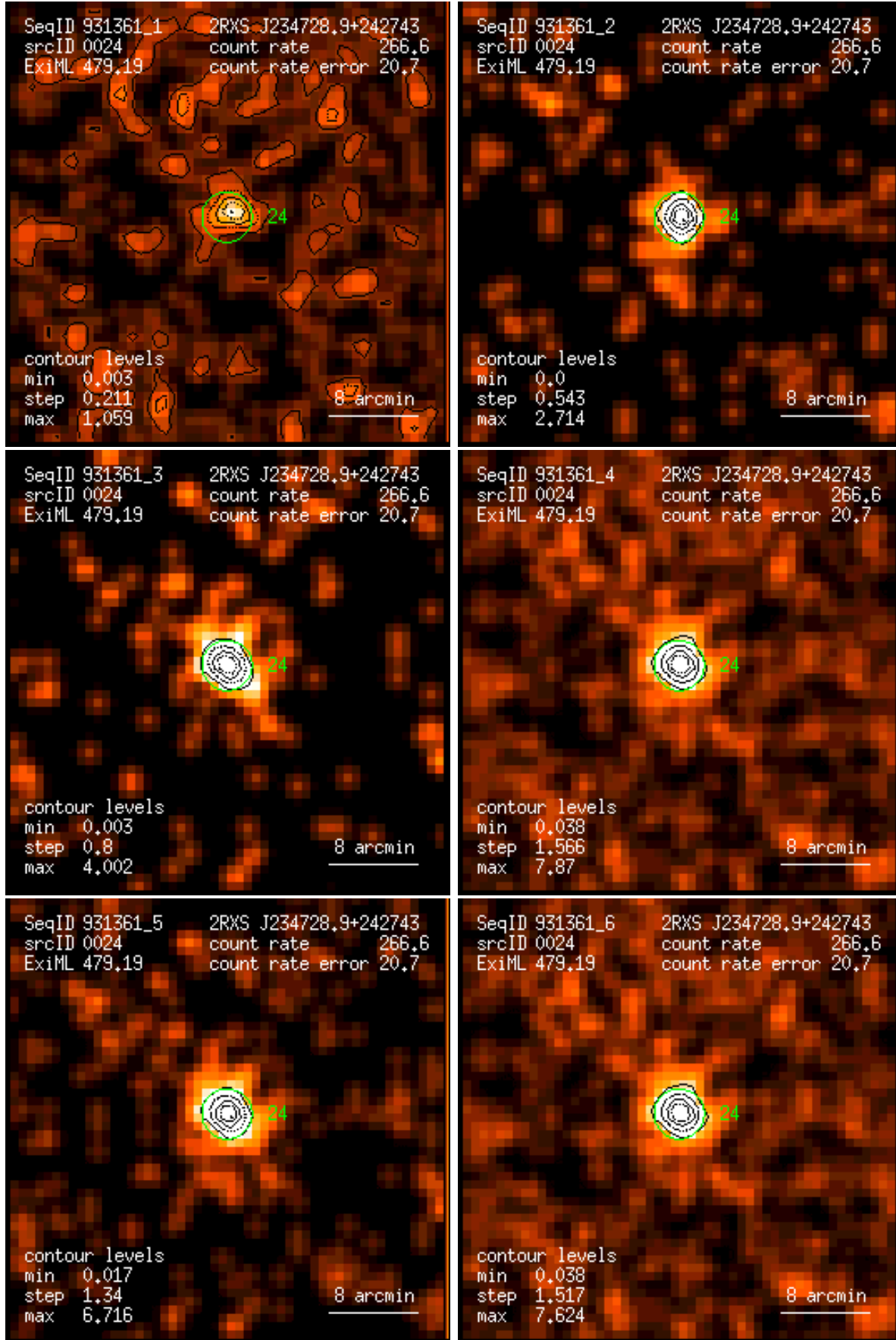
Figure 24: RASS 931361: detection 0024: band rate images, Gaussian filter: (1) PSPC channels 11 – 41, (2) 52 – 90, (3) 91 – 201, (4) 11 – 235, (5) 52 – 201, (6) 11 – 201. Broad band rates in counts/ks. Band rate contour levels in counts/ks/arcmin 2 .
