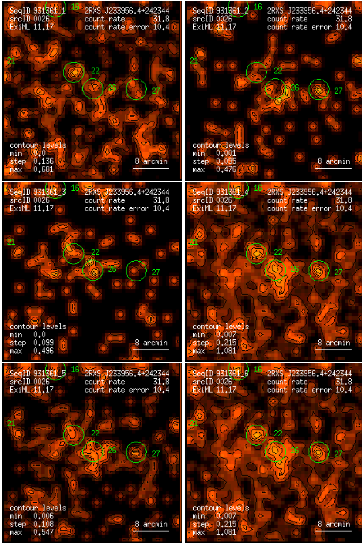
Figure 26: RASS 931361: detection 0026: band rate images, Gaussian filter: (1) PSPC channels 11 – 41, (2) 52 – 90, (3) 91 – 201, (4) 11 – 235, (5) 52 – 201, (6) 11 – 201. Broad band rates in counts/ks. Band rate contour levels in counts/ks/arcmin 2 .
