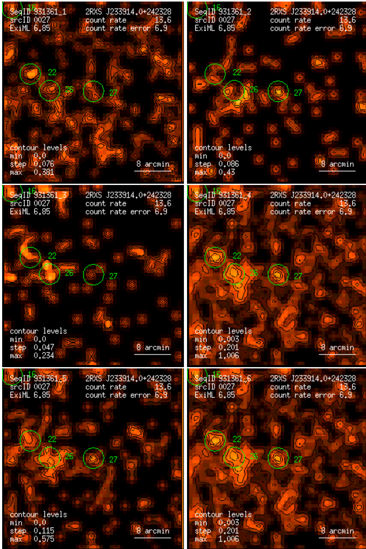
Figure 27: RASS 931361: detection 0027: band rate images, Gaussian filter: (1) PSPC channels 11 – 41, (2) 52 – 90, (3) 91 – 201, (4) 11 – 235, (5) 52 – 201, (6) 11 – 201. Broad band rates in counts/ks. Band rate contour levels in counts/ks/arcmin 2 .
