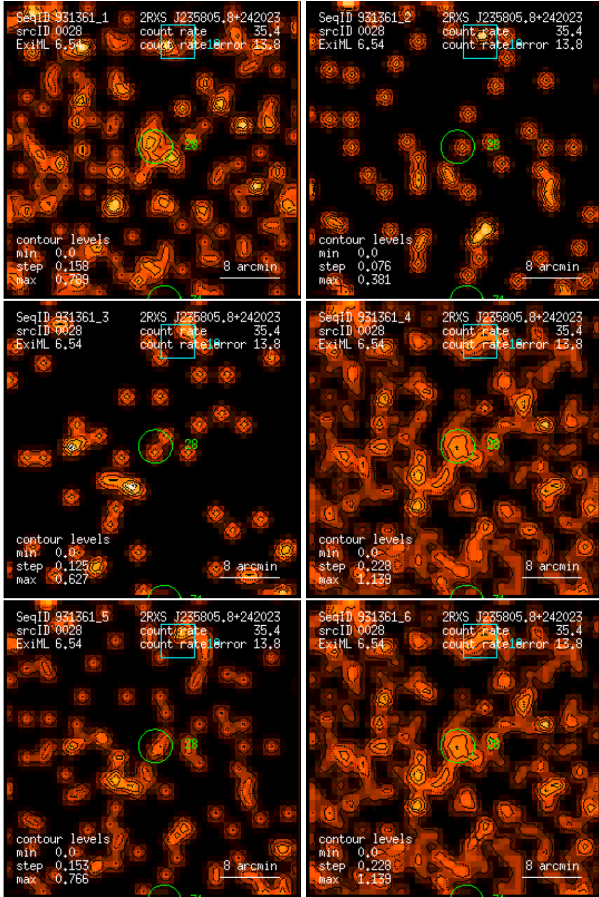
Figure 28: RASS 931361: detection 0028: band rate images, Gaussian filter: (1) PSPC channels 11 – 41, (2) 52 – 90, (3) 91 – 201, (4) 11 – 235, (5) 52 – 201, (6) 11 – 201. Broad band rates in counts/ks. Band rate contour levels in counts/ks/arcmin 2 .
