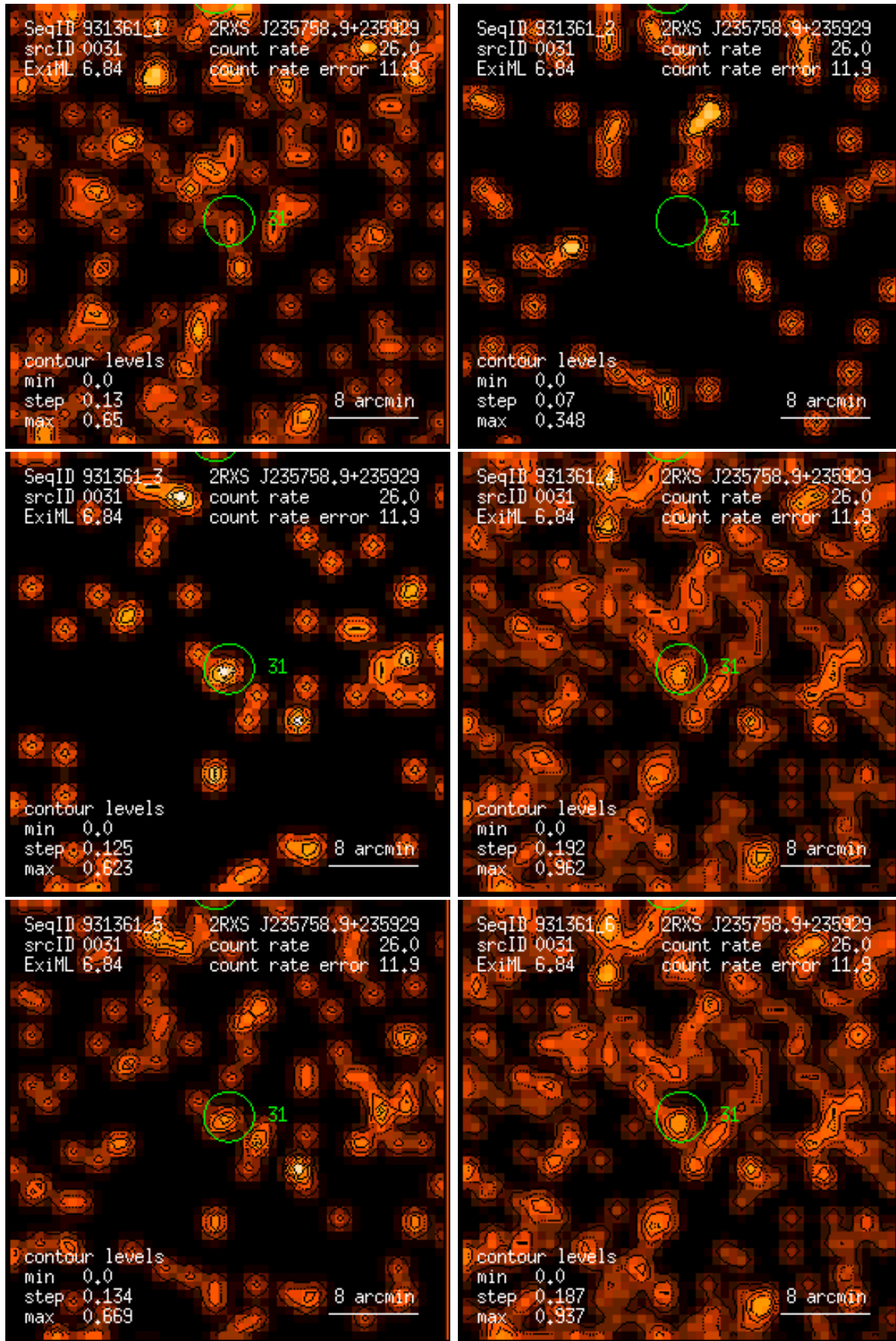
Figure 31: RASS 931361: detection 0031: band rate images, Gaussian filter: (1) PSPC channels 11 – 41, (2) 52 – 90, (3) 91 – 201, (4) 11 – 235, (5) 52 – 201, (6) 11 – 201. Broad band rates in counts/ks. Band rate contour levels in counts/ks/arcmin 2 .
