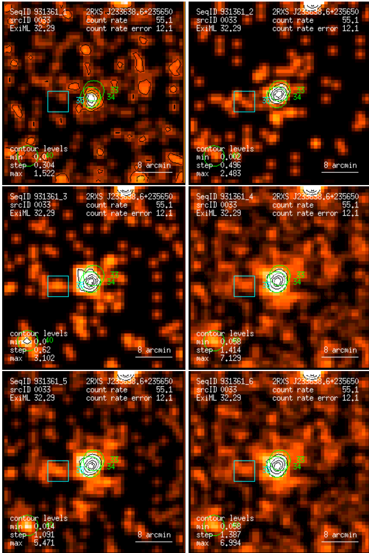
Figure 33: RASS 931361: detection 0033: band rate images, Gaussian filter: (1) PSPC channels 11 – 41, (2) 52 – 90, (3) 91 – 201, (4) 11 – 235, (5) 52 – 201, (6) 11 – 201. Broad band rates in counts/ks. Band rate contour levels in counts/ks/arcmin 2 .
