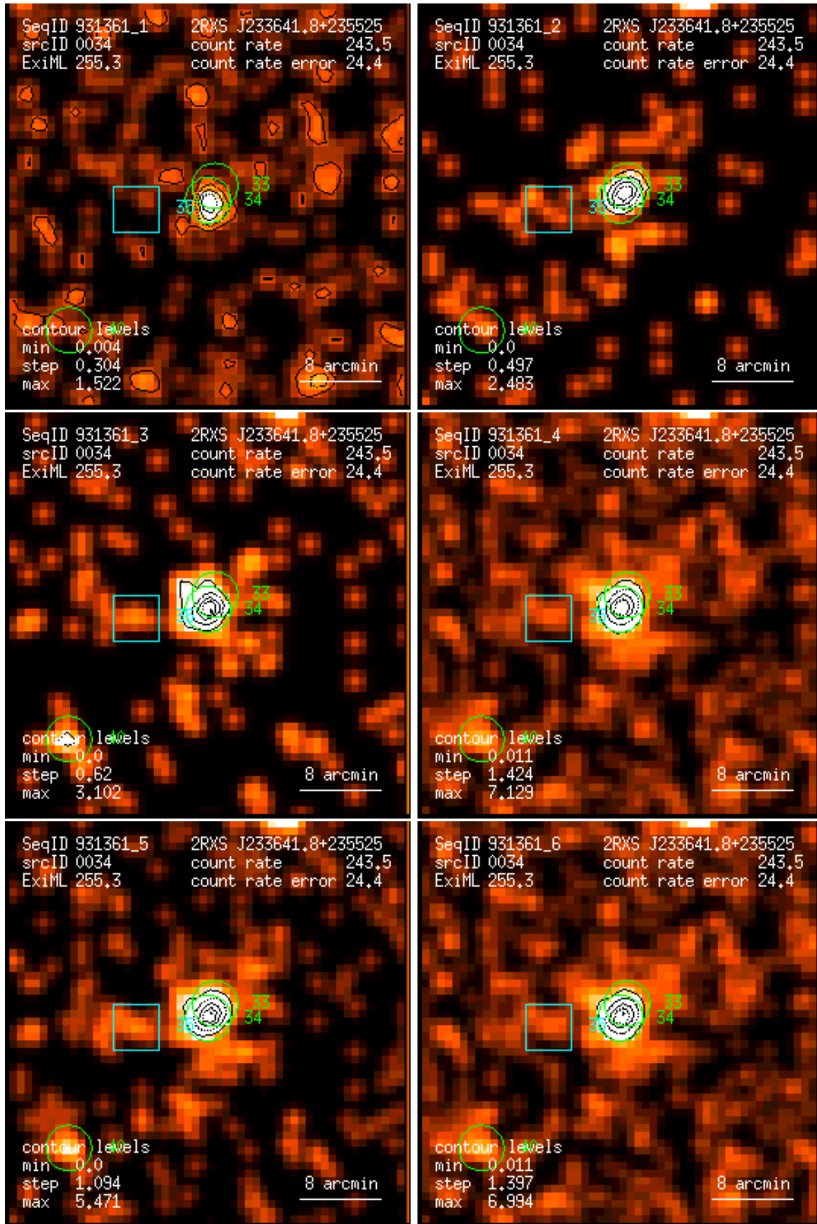
Figure 34: RASS 931361: detection 0034: band rate images, Gaussian filter: (1) PSPC channels 11 – 41, (2) 52 – 90, (3) 91 – 201, (4) 11 – 235, (5) 52 – 201, (6) 11 – 201. Broad band rates in counts/ks. Band rate contour levels in counts/ks/arcmin 2 .
