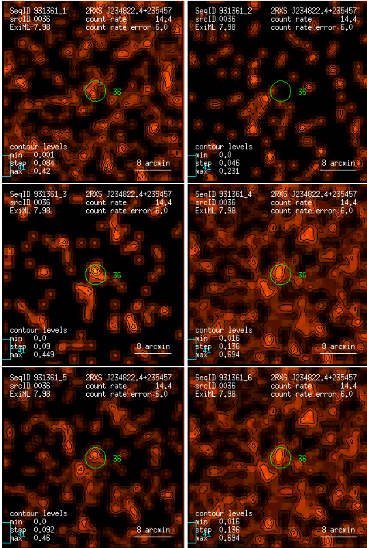
Figure 36: RASS 931361: detection 0036: band rate images, Gaussian filter: (1) PSPC channels 11 – 41, (2) 52 – 90, (3) 91 – 201, (4) 11 – 235, (5) 52 – 201, (6) 11 – 201. Broad band rates in counts/ks. Band rate contour levels in counts/ks/arcmin 2 .
