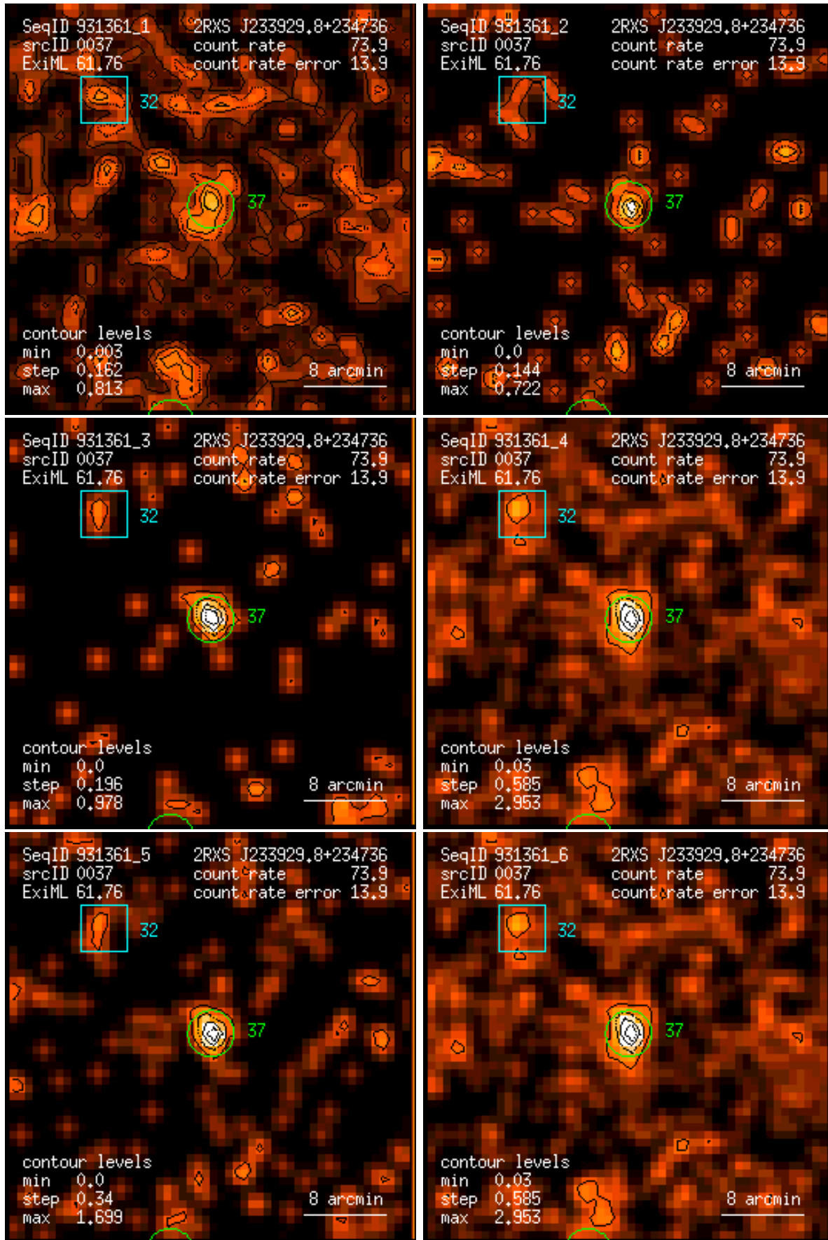
Figure 37: RASS 931361: detection 0037: band rate images, Gaussian filter: (1) PSPC channels 11 – 41, (2) 52 – 90, (3) 91 – 201, (4) 11 – 235, (5) 52 – 201, (6) 11 – 201. Broad band rates in counts/ks. Band rate contour levels in counts/ks/arcmin 2 .
