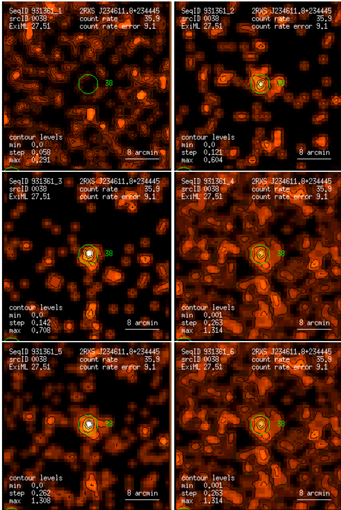
Figure 38: RASS 931361: detection 0038: band rate images, Gaussian filter: (1) PSPC channels 11 – 41, (2) 52 – 90, (3) 91 – 201, (4) 11 – 235, (5) 52 – 201, (6) 11 – 201. Broad band rates in counts/ks. Band rate contour levels in counts/ks/arcmin 2 .
