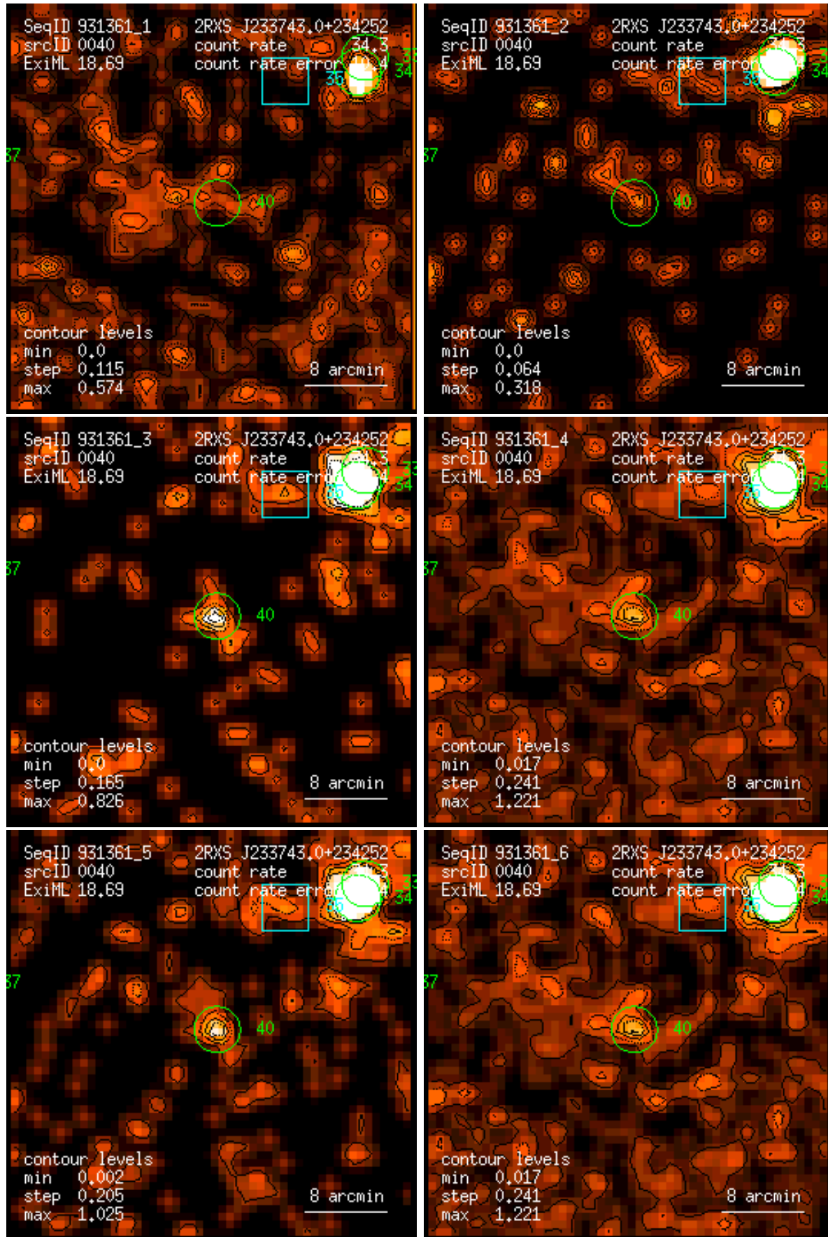
Figure 40: RASS 931361: detection 0040: band rate images, Gaussian filter: (1) PSPC channels 11 – 41, (2) 52 – 90, (3) 91 – 201, (4) 11 – 235, (5) 52 – 201, (6) 11 – 201. Broad band rates in counts/ks. Band rate contour levels in counts/ks/arcmin 2 .
