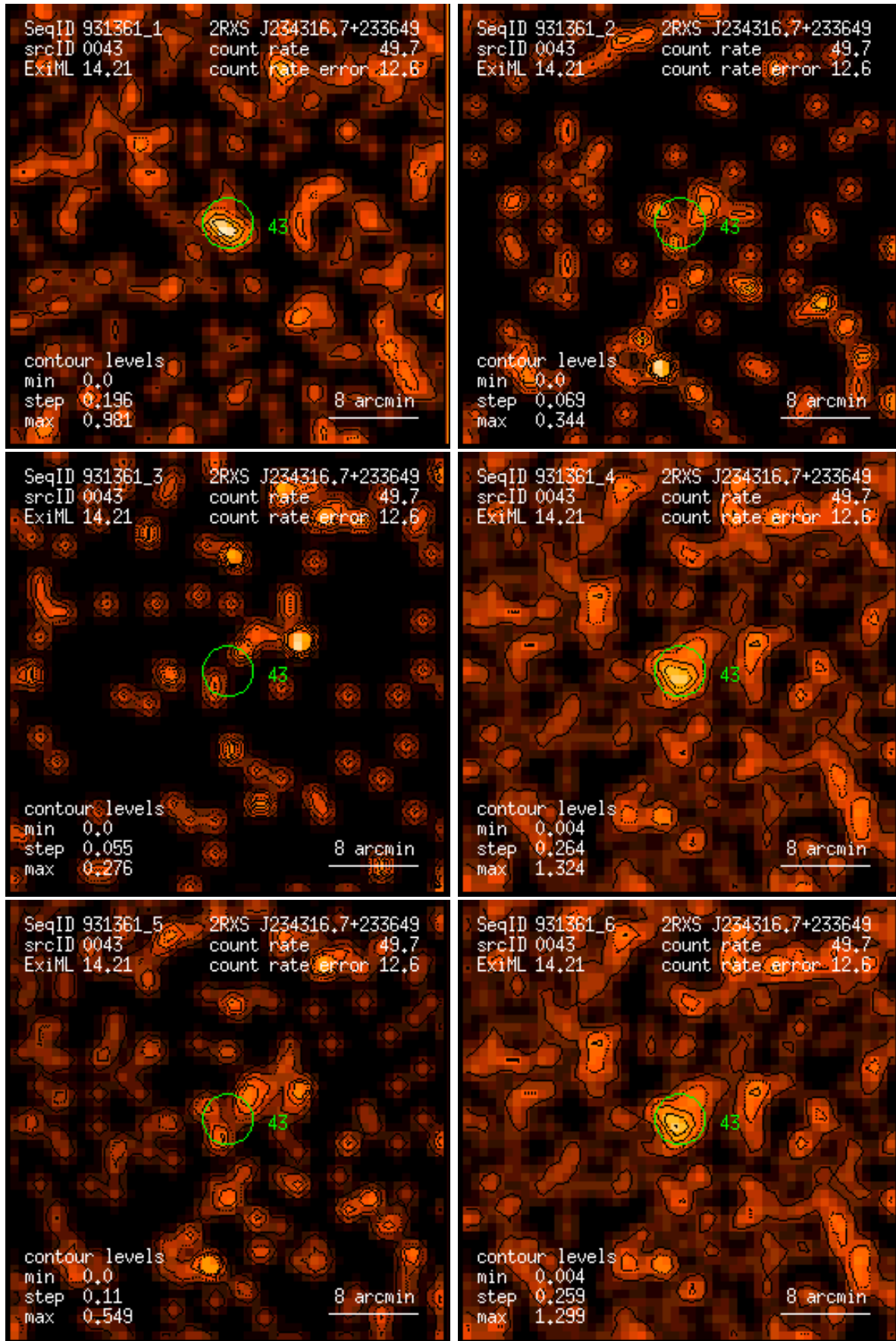
Figure 43: RASS 931361: detection 0043: band rate images, Gaussian filter: (1) PSPC channels 11 – 41, (2) 52 – 90, (3) 91 – 201, (4) 11 – 235, (5) 52 – 201, (6) 11 – 201. Broad band rates in counts/ks. Band rate contour levels in counts/ks/arcmin 2 .
