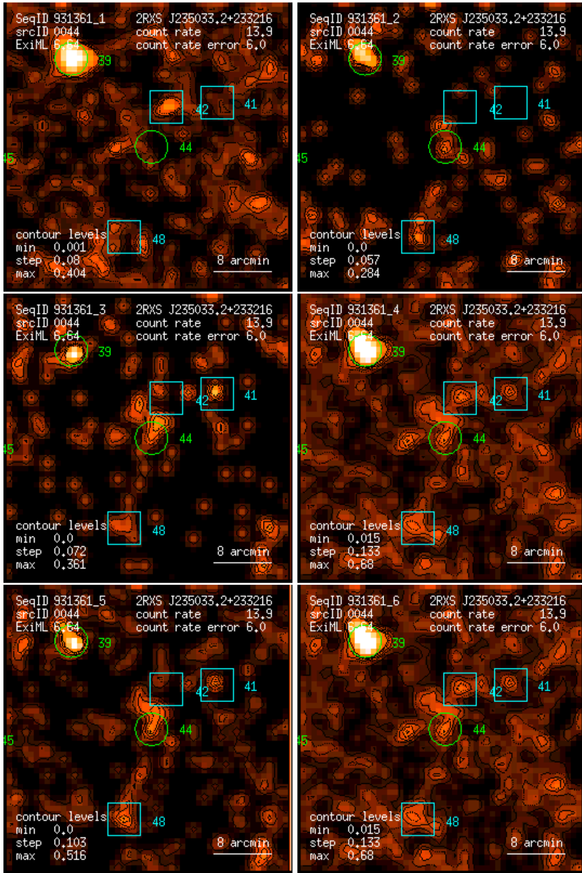
Figure 44: RASS 931361: detection 0044: band rate images, Gaussian filter: (1) PSPC channels 11 – 41, (2) 52 – 90, (3) 91 – 201, (4) 11 – 235, (5) 52 – 201, (6) 11 – 201. Broad band rates in counts/ks. Band rate contour levels in counts/ks/arcmin 2 .
