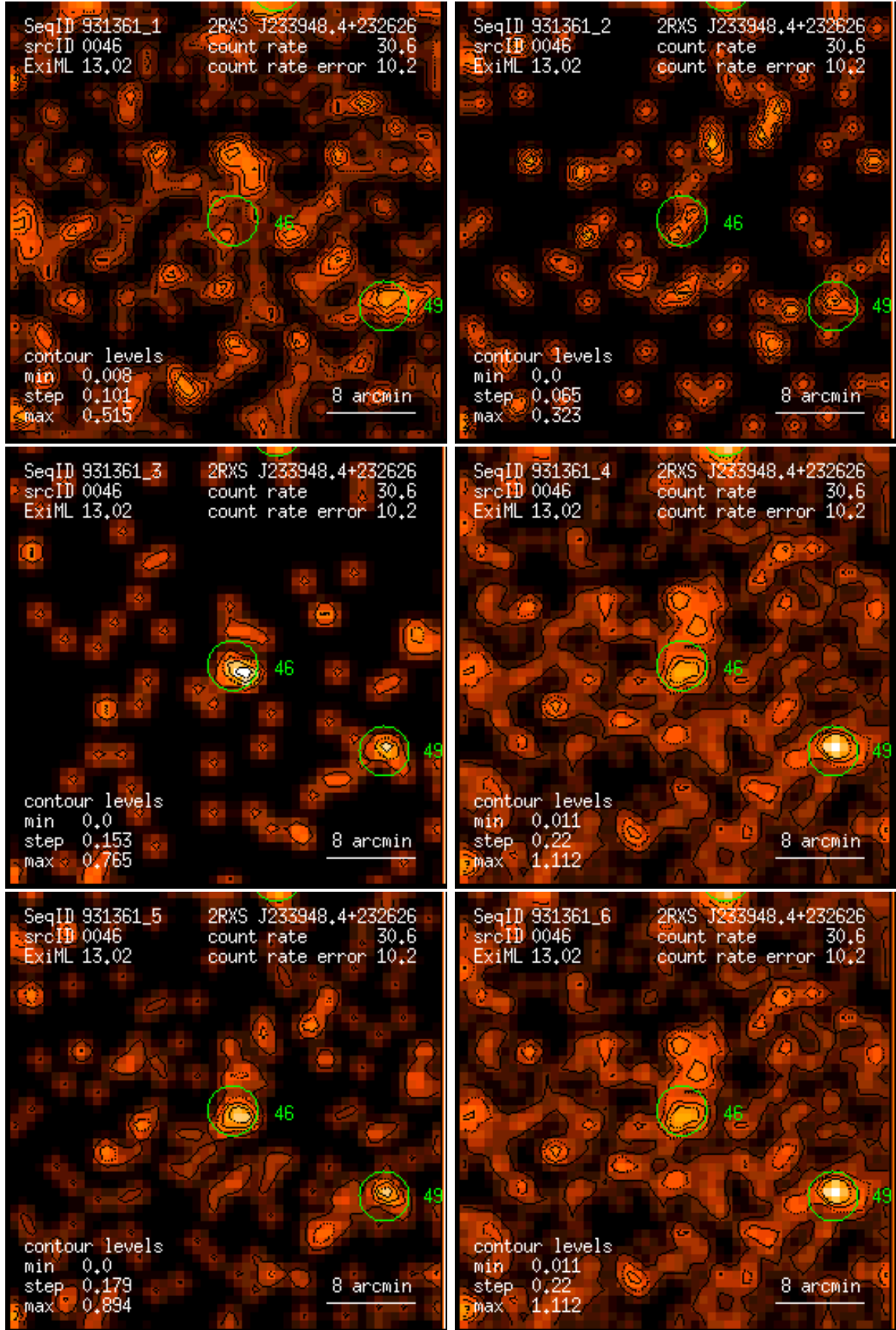
Figure 46: RASS 931361: detection 0046: band rate images, Gaussian filter: (1) PSPC channels 11 – 41, (2) 52 – 90, (3) 91 – 201, (4) 11 – 235, (5) 52 – 201, (6) 11 – 201. Broad band rates in counts/ks. Band rate contour levels in counts/ks/arcmin 2 .
