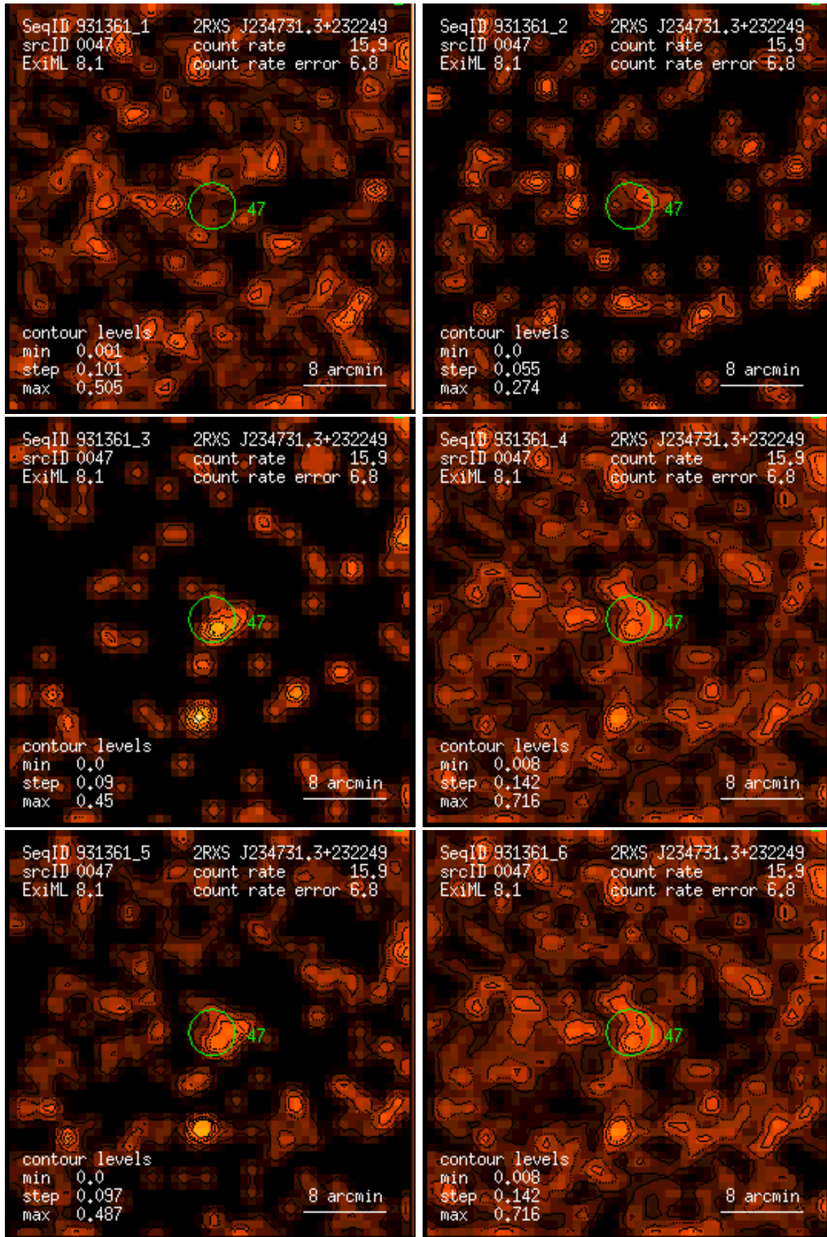
Figure 47: RASS 931361: detection 0047: band rate images, Gaussian filter: (1) PSPC channels 11 – 41, (2) 52 – 90, (3) 91 – 201, (4) 11 – 235, (5) 52 – 201, (6) 11 – 201. Broad band rates in counts/ks. Band rate contour levels in counts/ks/arcmin 2 .
