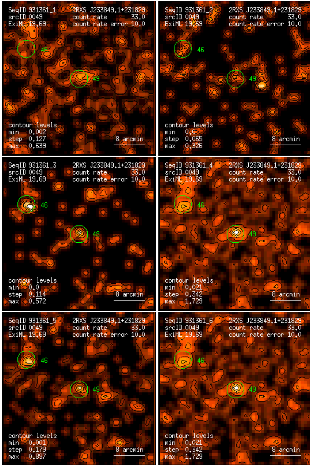
Figure 49: RASS 931361: detection 0049: band rate images, Gaussian filter: (1) PSPC channels 11 – 41, (2) 52 – 90, (3) 91 – 201, (4) 11 – 235, (5) 52 – 201, (6) 11 – 201. Broad band rates in counts/ks. Band rate contour levels in counts/ks/arcmin 2 .
