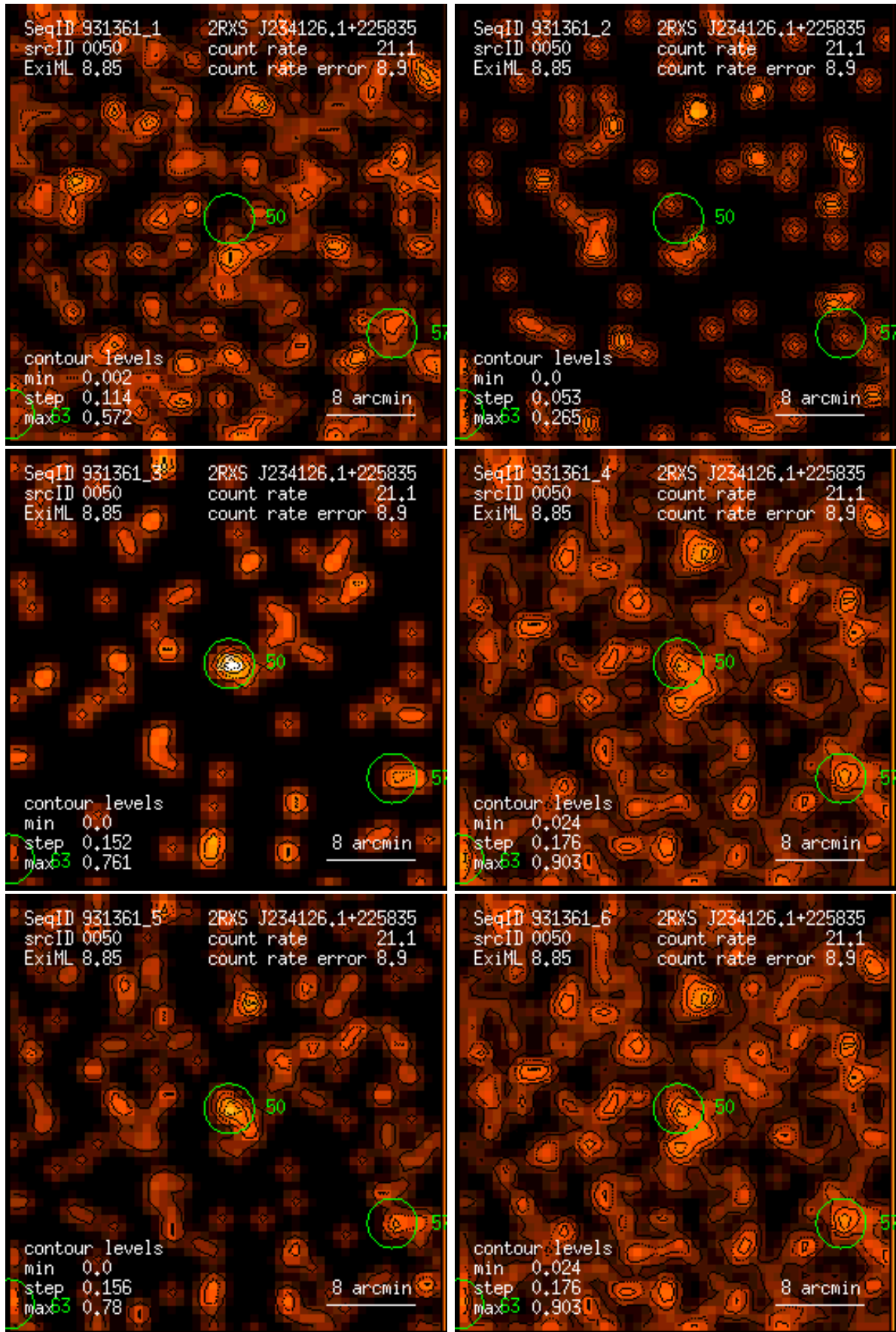
Figure 50: RASS 931361: detection 0050: band rate images, Gaussian filter: (1) PSPC channels 11 – 41, (2) 52 – 90, (3) 91 – 201, (4) 11 – 235, (5) 52 – 201, (6) 11 – 201. Broad band rates in counts/ks. Band rate contour levels in counts/ks/arcmin 2 .
