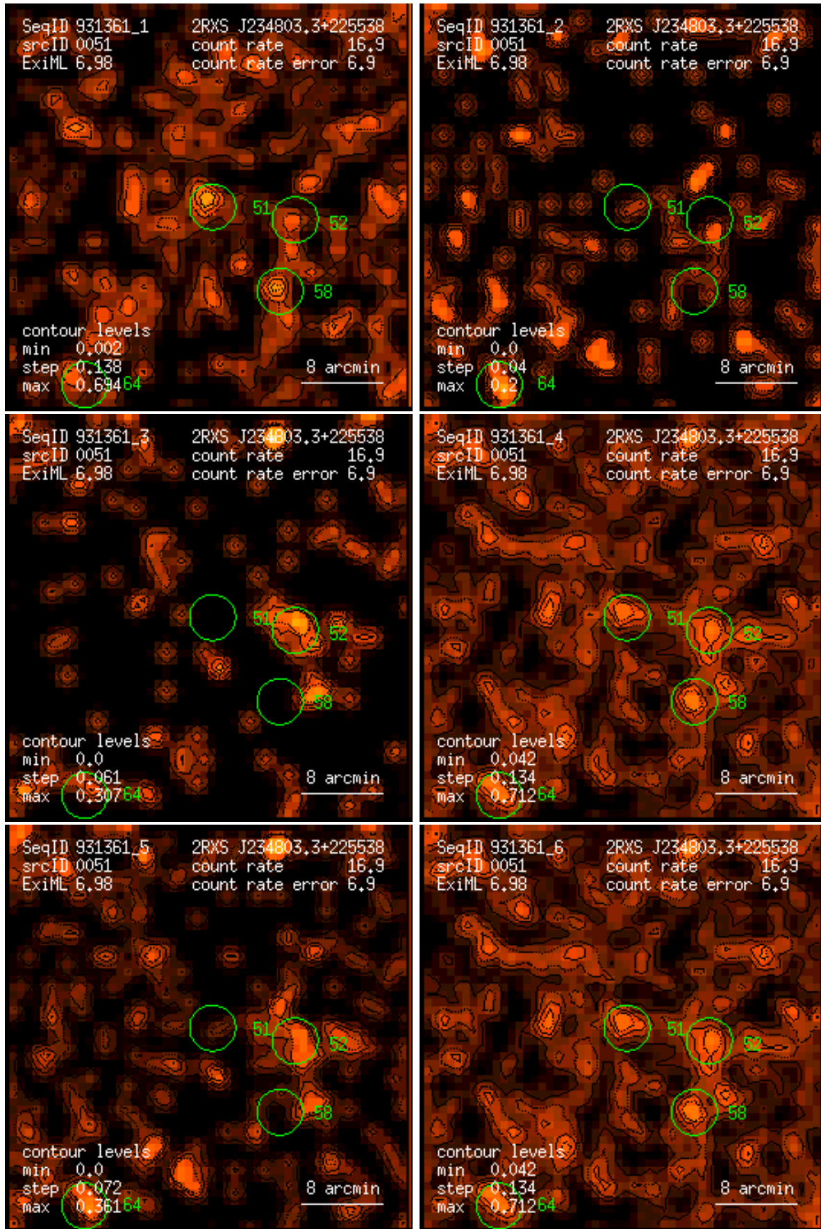
Figure 51: RASS 931361: detection 0051: band rate images, Gaussian filter: (1) PSPC channels 11 – 41, (2) 52 – 90, (3) 91 – 201, (4) 11 – 235, (5) 52 – 201, (6) 11 – 201. Broad band rates in counts/ks. Band rate contour levels in counts/ks/arcmin 2 .
