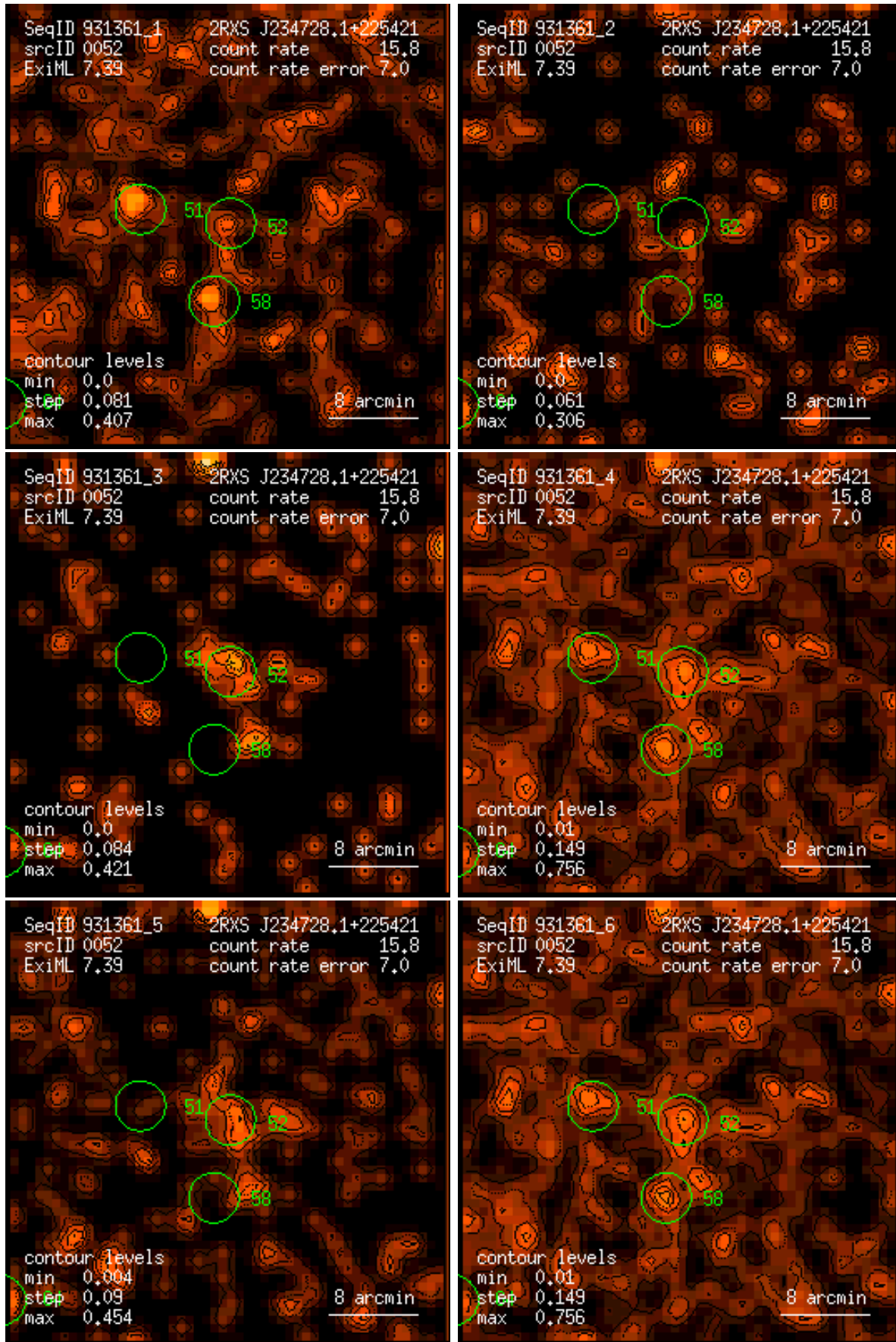
Figure 52: RASS 931361: detection 0052: band rate images, Gaussian filter: (1) PSPC channels 11 – 41, (2) 52 – 90, (3) 91 – 201, (4) 11 – 235, (5) 52 – 201, (6) 11 – 201. Broad band rates in counts/ks. Band rate contour levels in counts/ks/arcmin 2 .
