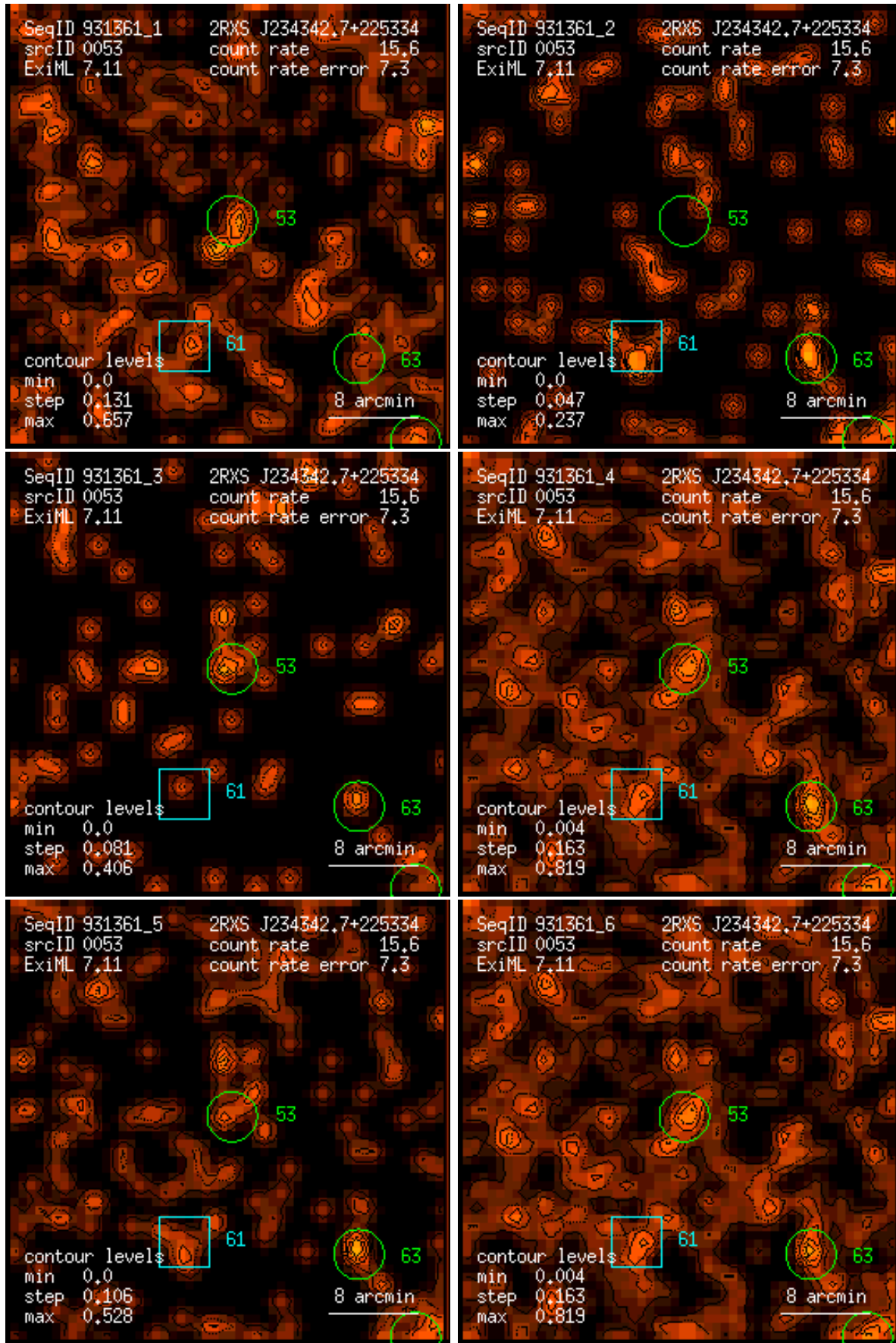
Figure 53: RASS 931361: detection 0053: band rate images, Gaussian filter: (1) PSPC channels 11 – 41, (2) 52 – 90, (3) 91 – 201, (4) 11 – 235, (5) 52 – 201, (6) 11 – 201. Broad band rates in counts/ks. Band rate contour levels in counts/ks/arcmin 2 .
