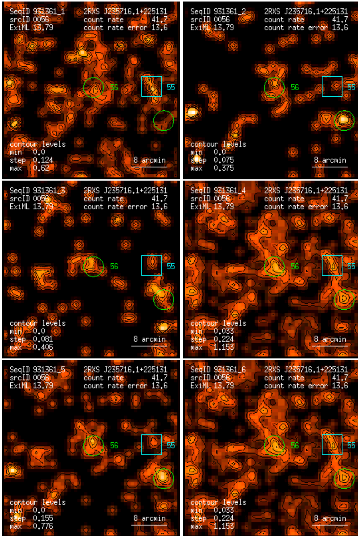
Figure 56: RASS 931361: detection 0056: band rate images, Gaussian filter: (1) PSPC channels 11 – 41, (2) 52 – 90, (3) 91 – 201, (4) 11 – 235, (5) 52 – 201, (6) 11 – 201. Broad band rates in counts/ks. Band rate contour levels in counts/ks/arcmin 2 .
