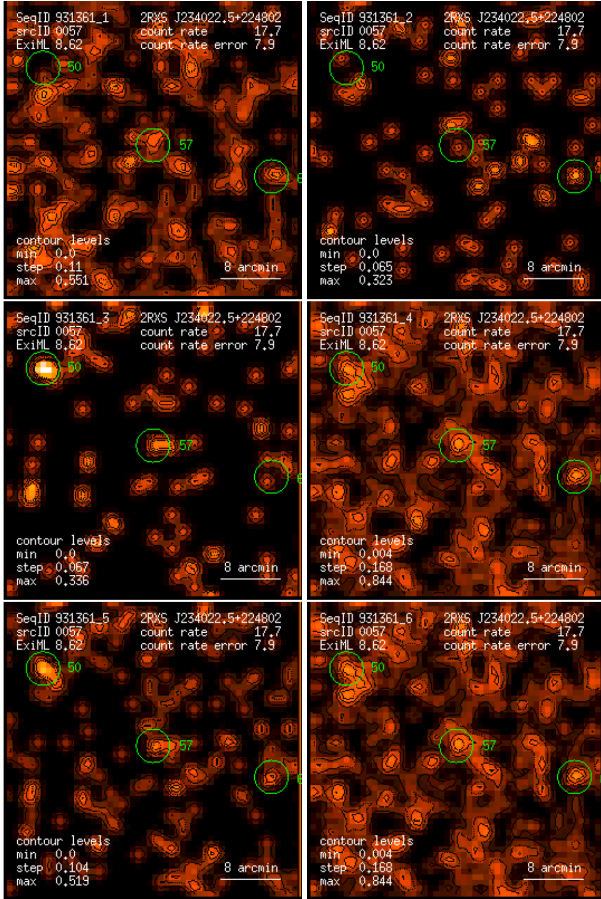
Figure 57: RASS 931361: detection 0057: band rate images, Gaussian filter: (1) PSPC channels 11 – 41, (2) 52 – 90, (3) 91 – 201, (4) 11 – 235, (5) 52 – 201, (6) 11 – 201. Broad band rates in counts/ks. Band rate contour levels in counts/ks/arcmin 2 .
