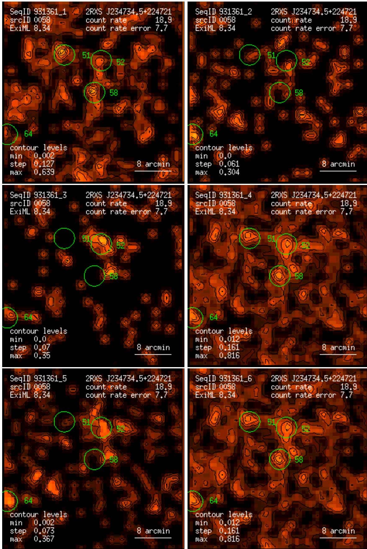
Figure 58: RASS 931361: detection 0058: band rate images, Gaussian filter: (1) PSPC channels 11 – 41, (2) 52 – 90, (3) 91 – 201, (4) 11 – 235, (5) 52 – 201, (6) 11 – 201. Broad band rates in counts/ks. Band rate contour levels in counts/ks/arcmin 2 .
