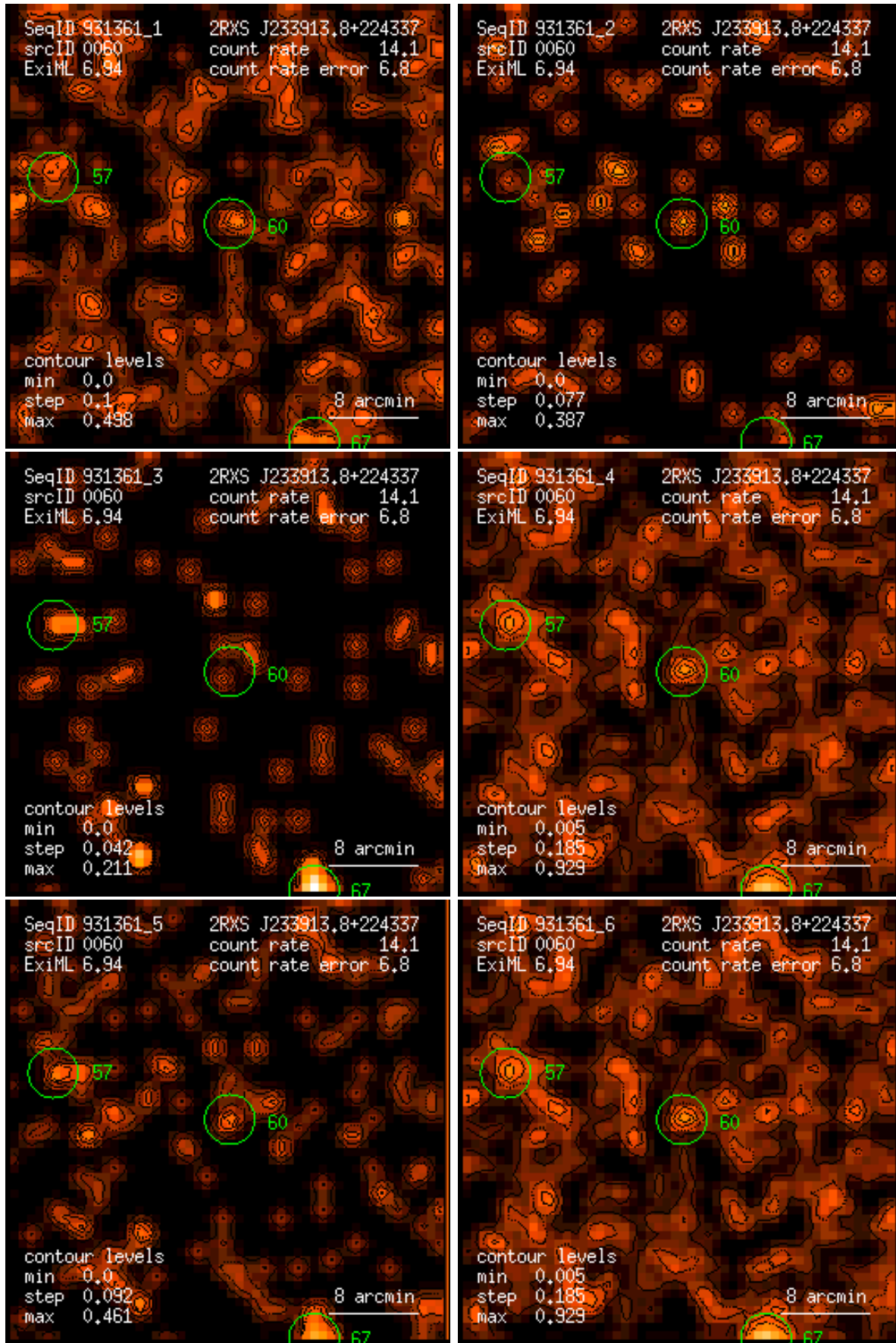
Figure 60: RASS 931361: detection 0060: band rate images, Gaussian filter: (1) PSPC channels 11 – 41, (2) 52 – 90, (3) 91 – 201, (4) 11 – 235, (5) 52 – 201, (6) 11 – 201. Broad band rates in counts/ks. Band rate contour levels in counts/ks/arcmin 2 .
