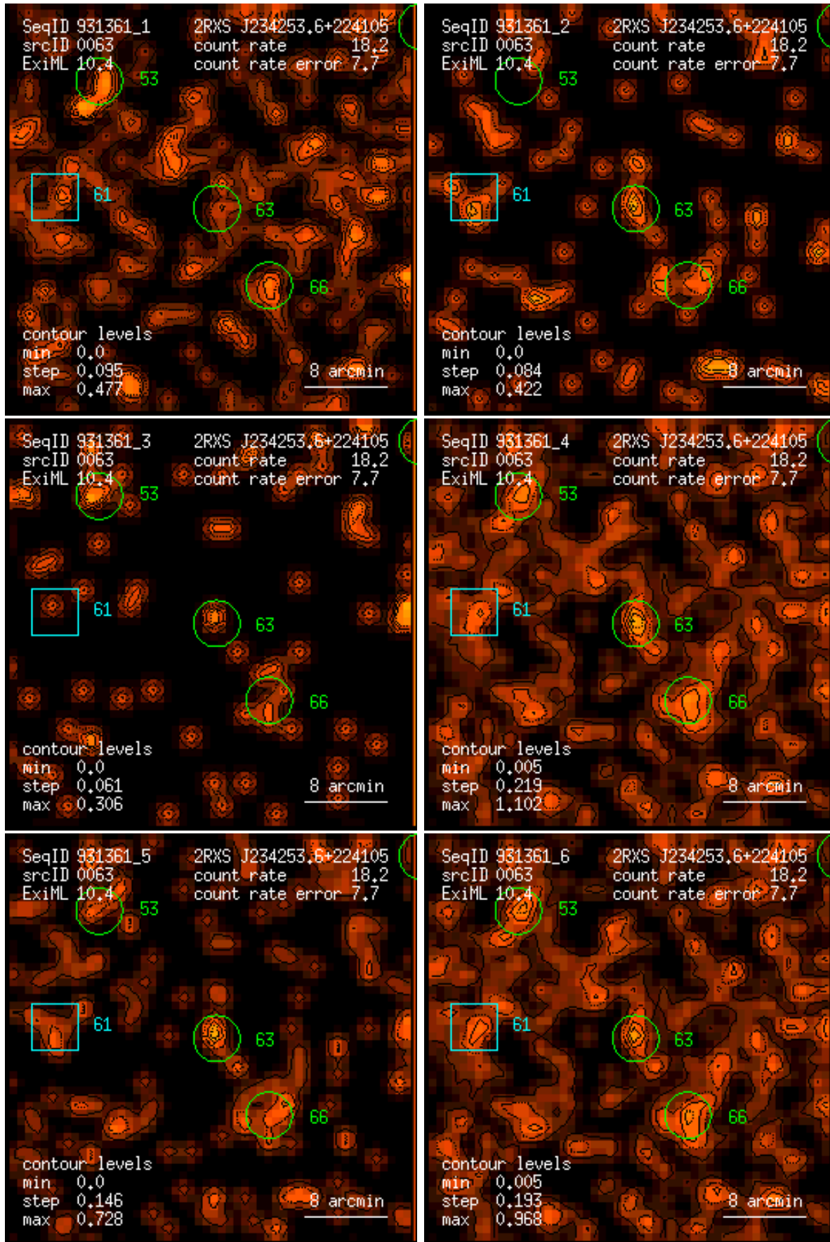
Figure 63: RASS 931361: detection 0063: band rate images, Gaussian filter: (1) PSPC channels 11 – 41, (2) 52 – 90, (3) 91 – 201, (4) 11 – 235, (5) 52 – 201, (6) 11 – 201. Broad band rates in counts/ks. Band rate contour levels in counts/ks/arcmin 2 .
