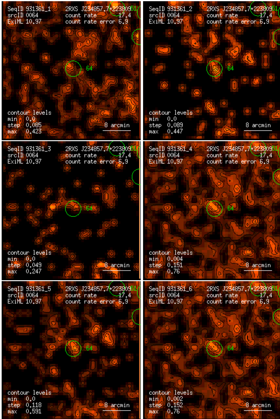
Figure 64: RASS 931361: detection 0064: band rate images, Gaussian filter: (1) PSPC channels 11 – 41, (2) 52 – 90, (3) 91 – 201, (4) 11 – 235, (5) 52 – 201, (6) 11 – 201. Broad band rates in counts/ks. Band rate contour levels in counts/ks/arcmin 2 .
