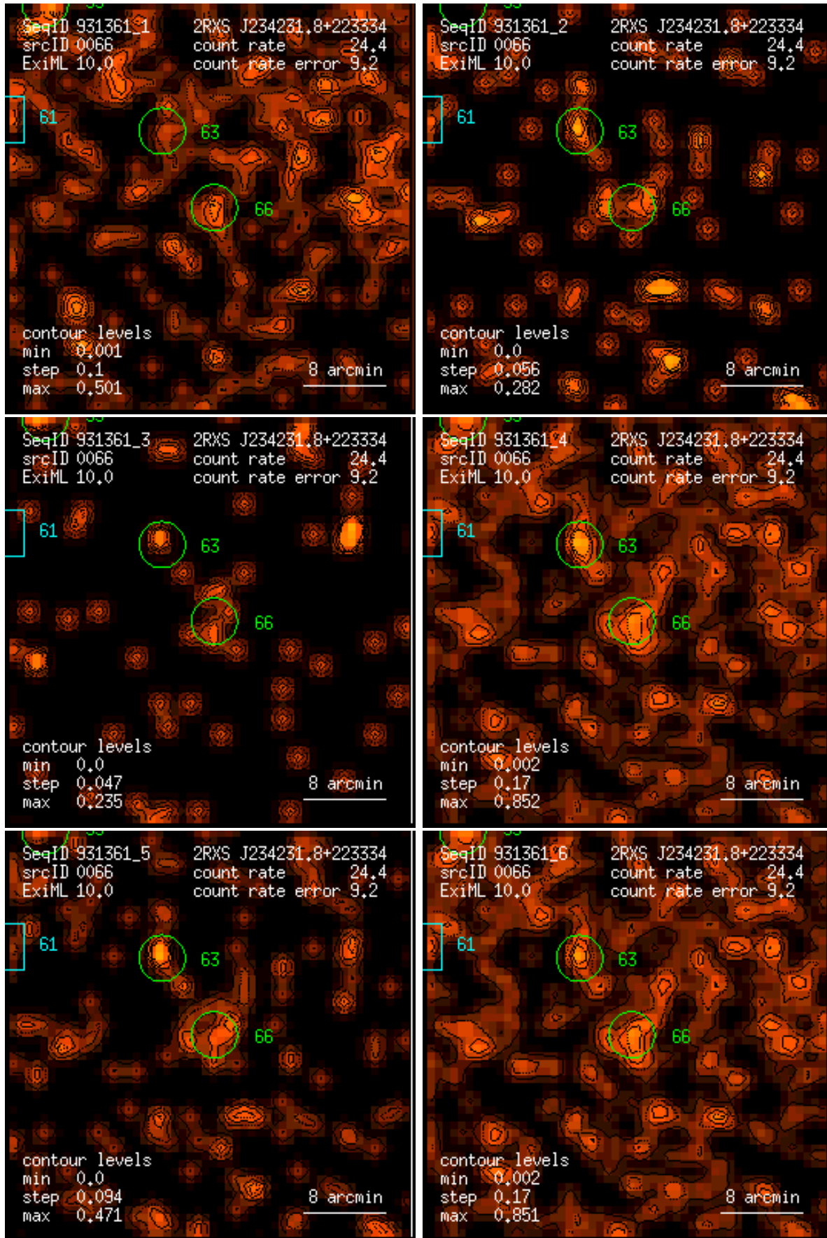
Figure 66: RASS 931361: detection 0066: band rate images, Gaussian filter: (1) PSPC channels 11 – 41, (2) 52 – 90, (3) 91 – 201, (4) 11 – 235, (5) 52 – 201, (6) 11 – 201. Broad band rates in counts/ks. Band rate contour levels in counts/ks/arcmin 2 .
