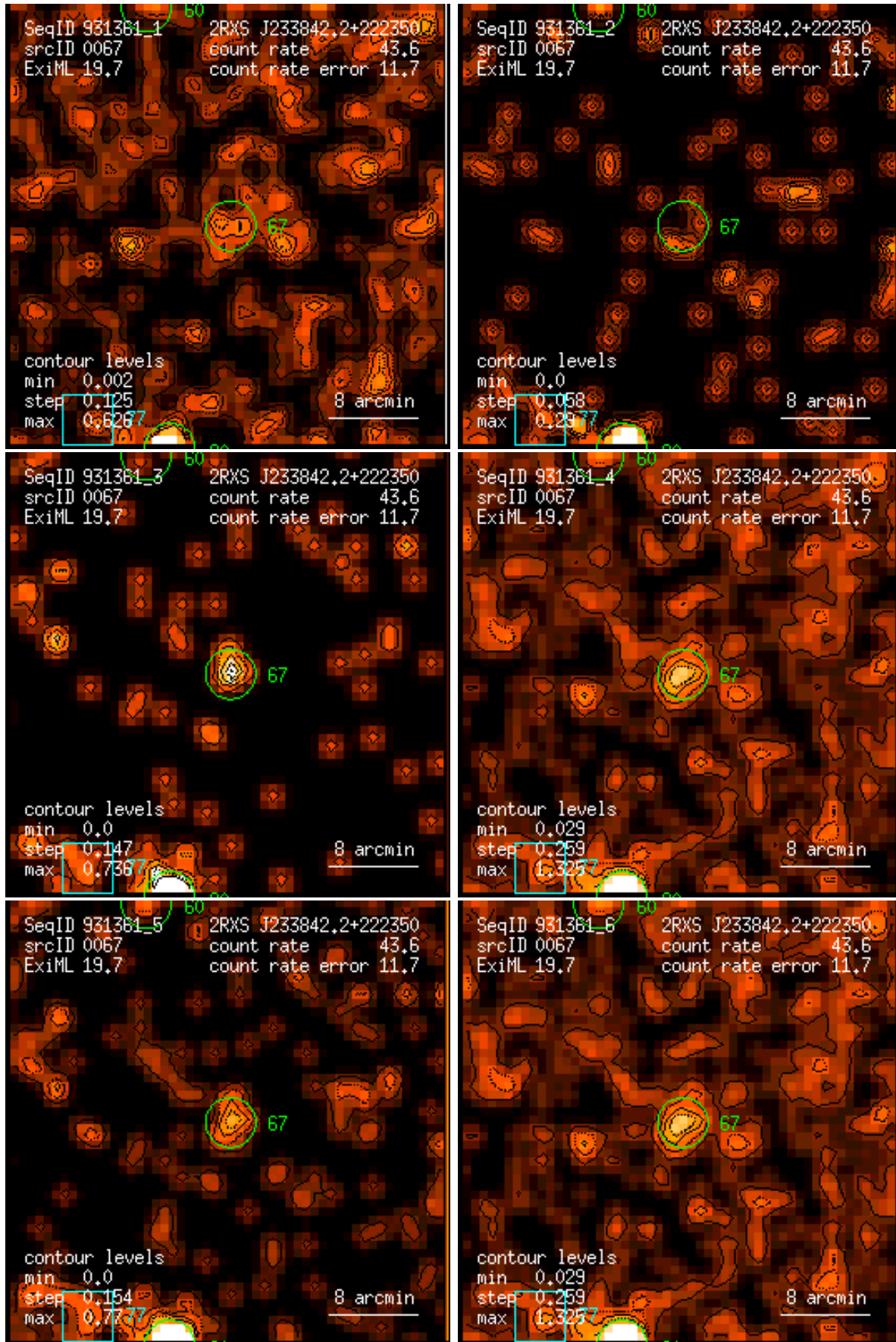
Figure 67: RASS 931361: detection 0067: band rate images, Gaussian filter: (1) PSPC channels 11 – 41, (2) 52 – 90, (3) 91 – 201, (4) 11 – 235, (5) 52 – 201, (6) 11 – 201. Broad band rates in counts/ks. Band rate contour levels in counts/ks/arcmin 2 .
