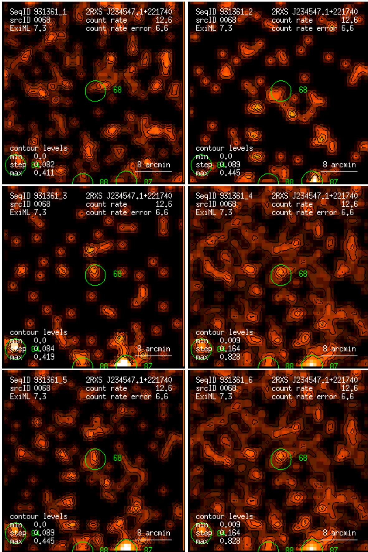
Figure 68: RASS 931361: detection 0068: band rate images, Gaussian filter: (1) PSPC channels 11 – 41, (2) 52 – 90, (3) 91 – 201, (4) 11 – 235, (5) 52 – 201, (6) 11 – 201. Broad band rates in counts/ks. Band rate contour levels in counts/ks/arcmin 2 .
