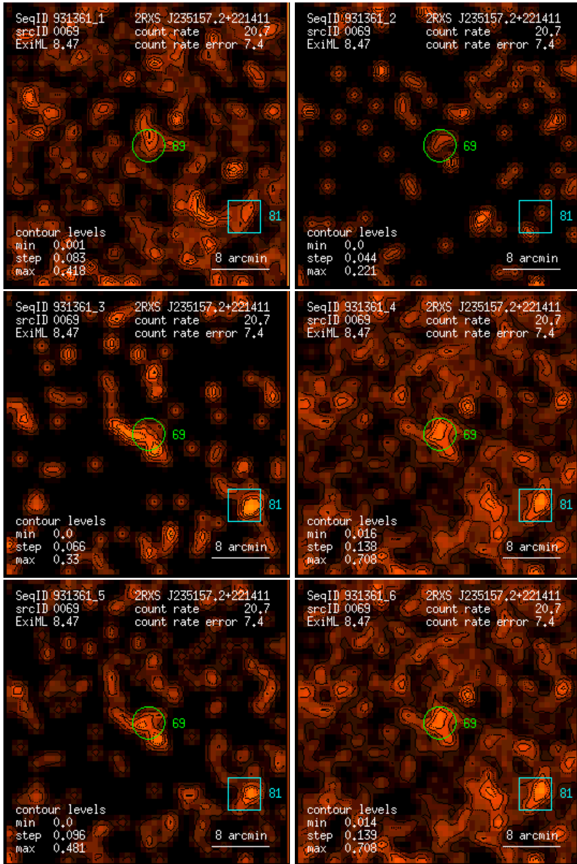
Figure 69: RASS 931361: detection 0069: band rate images, Gaussian filter: (1) PSPC channels 11 – 41, (2) 52 – 90, (3) 91 – 201, (4) 11 – 235, (5) 52 – 201, (6) 11 – 201. Broad band rates in counts/ks. Band rate contour levels in counts/ks/arcmin 2 .
