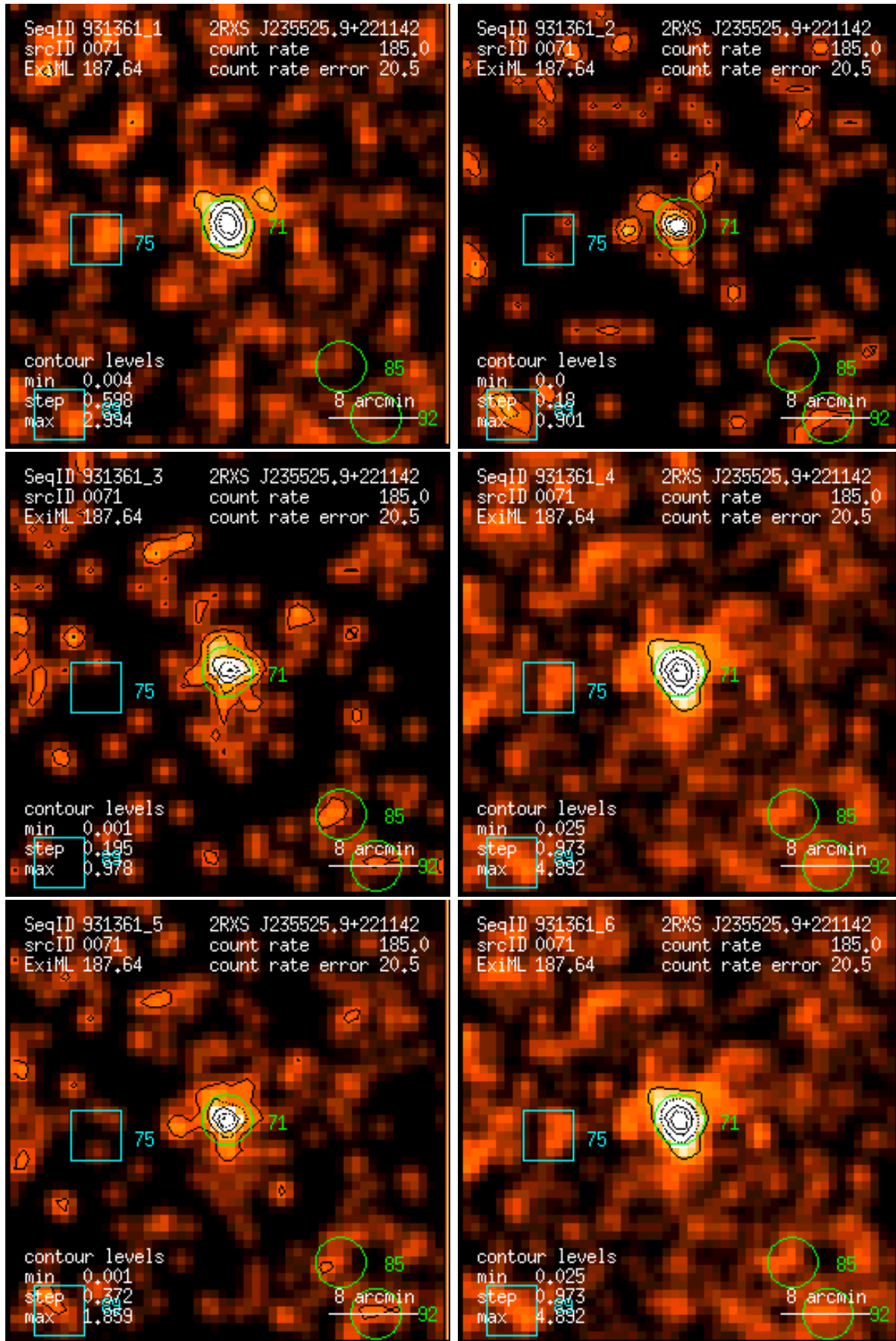
Figure 71: RASS 931361: detection 0071: band rate images, Gaussian filter: (1) PSPC channels 11 – 41, (2) 52 – 90, (3) 91 – 201, (4) 11 – 235, (5) 52 – 201, (6) 11 – 201. Broad band rates in counts/ks. Band rate contour levels in counts/ks/arcmin 2 .
