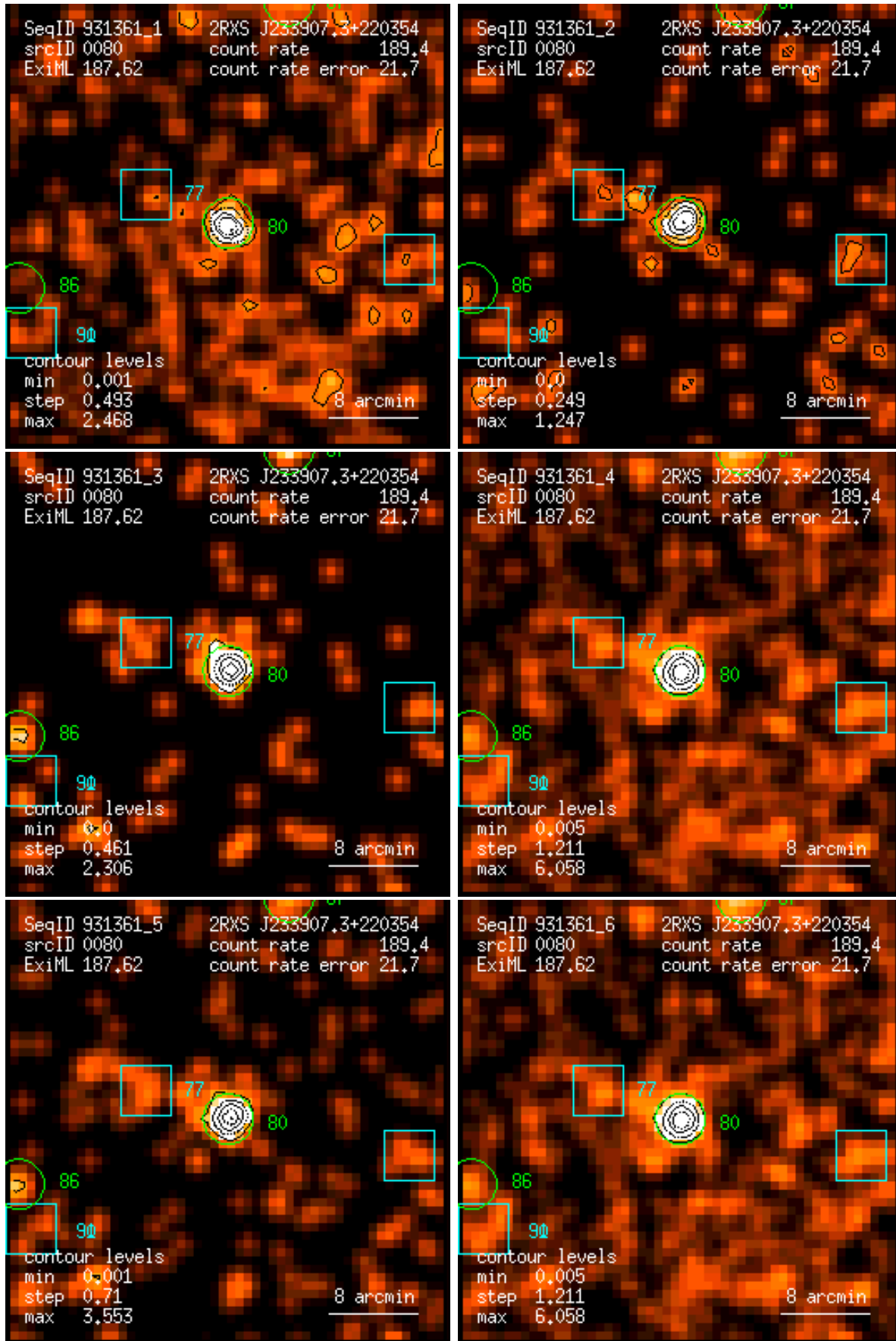
Figure 80: RASS 931361: detection 0080: band rate images, Gaussian filter: (1) PSPC channels 11 – 41, (2) 52 – 90, (3) 91 – 201, (4) 11 – 235, (5) 52 – 201, (6) 11 – 201. Broad band rates in counts/ks. Band rate contour levels in counts/ks/arcmin 2 .
