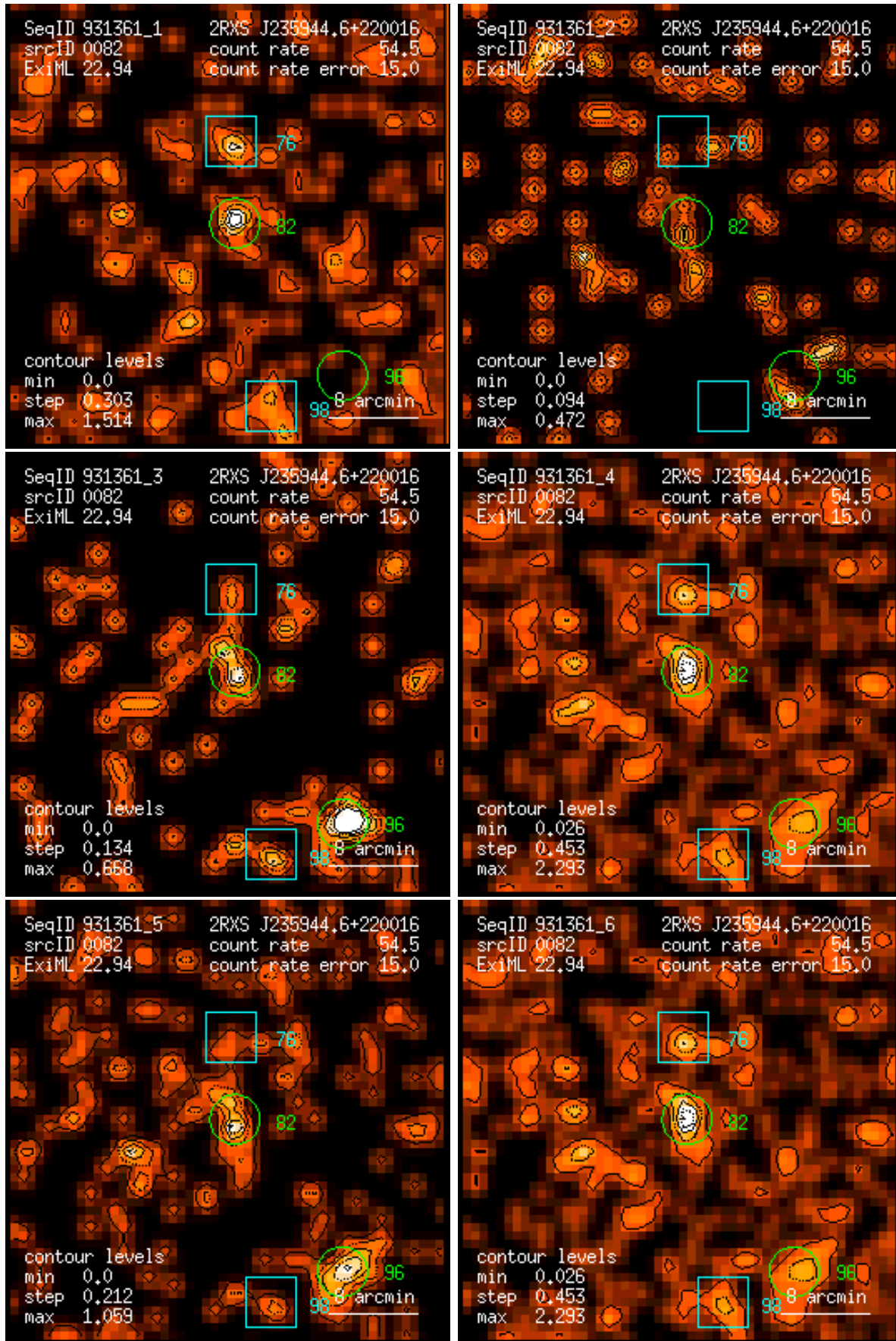
Figure 82: RASS 931361: detection 0082: band rate images, Gaussian filter: (1) PSPC channels 11 – 41, (2) 52 – 90, (3) 91 – 201, (4) 11 – 235, (5) 52 – 201, (6) 11 – 201. Broad band rates in counts/ks. Band rate contour levels in counts/ks/arcmin 2 .
