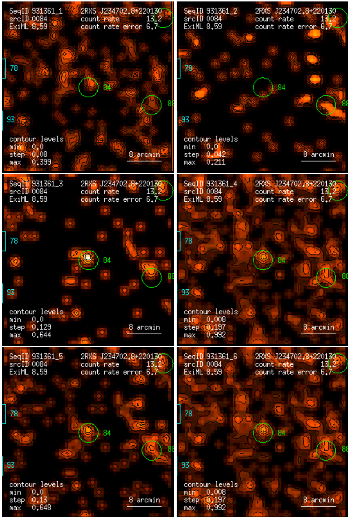
Figure 84: RASS 931361: detection 0084: band rate images, Gaussian filter: (1) PSPC channels 11 – 41, (2) 52 – 90, (3) 91 – 201, (4) 11 – 235, (5) 52 – 201, (6) 11 – 201. Broad band rates in counts/ks. Band rate contour levels in counts/ks/arcmin 2 .
