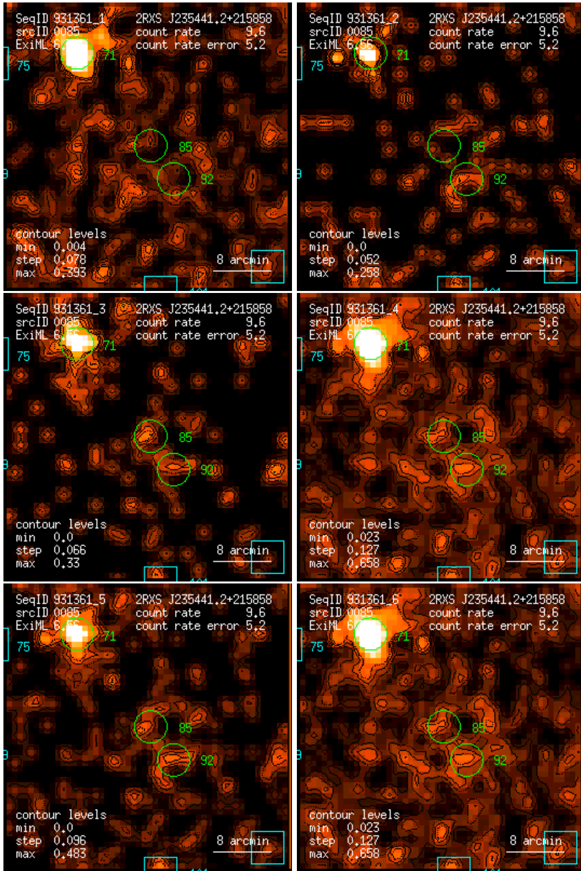
Figure 85: RASS 931361: detection 0085: band rate images, Gaussian filter: (1) PSPC channels 11 – 41, (2) 52 – 90, (3) 91 – 201, (4) 11 – 235, (5) 52 – 201, (6) 11 – 201. Broad band rates in counts/ks. Band rate contour levels in counts/ks/arcmin 2 .
