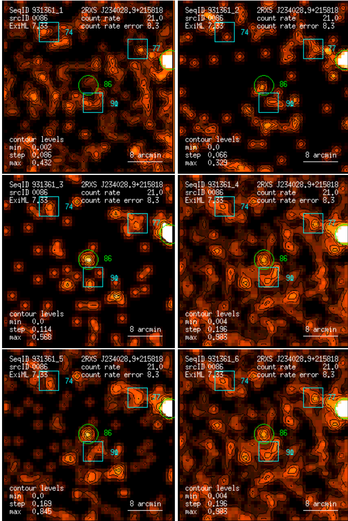
Figure 86: RASS 931361: detection 0086: band rate images, Gaussian filter: (1) PSPC channels 11 – 41, (2) 52 – 90, (3) 91 – 201, (4) 11 – 235, (5) 52 – 201, (6) 11 – 201. Broad band rates in counts/ks. Band rate contour levels in counts/ks/arcmin 2 .
