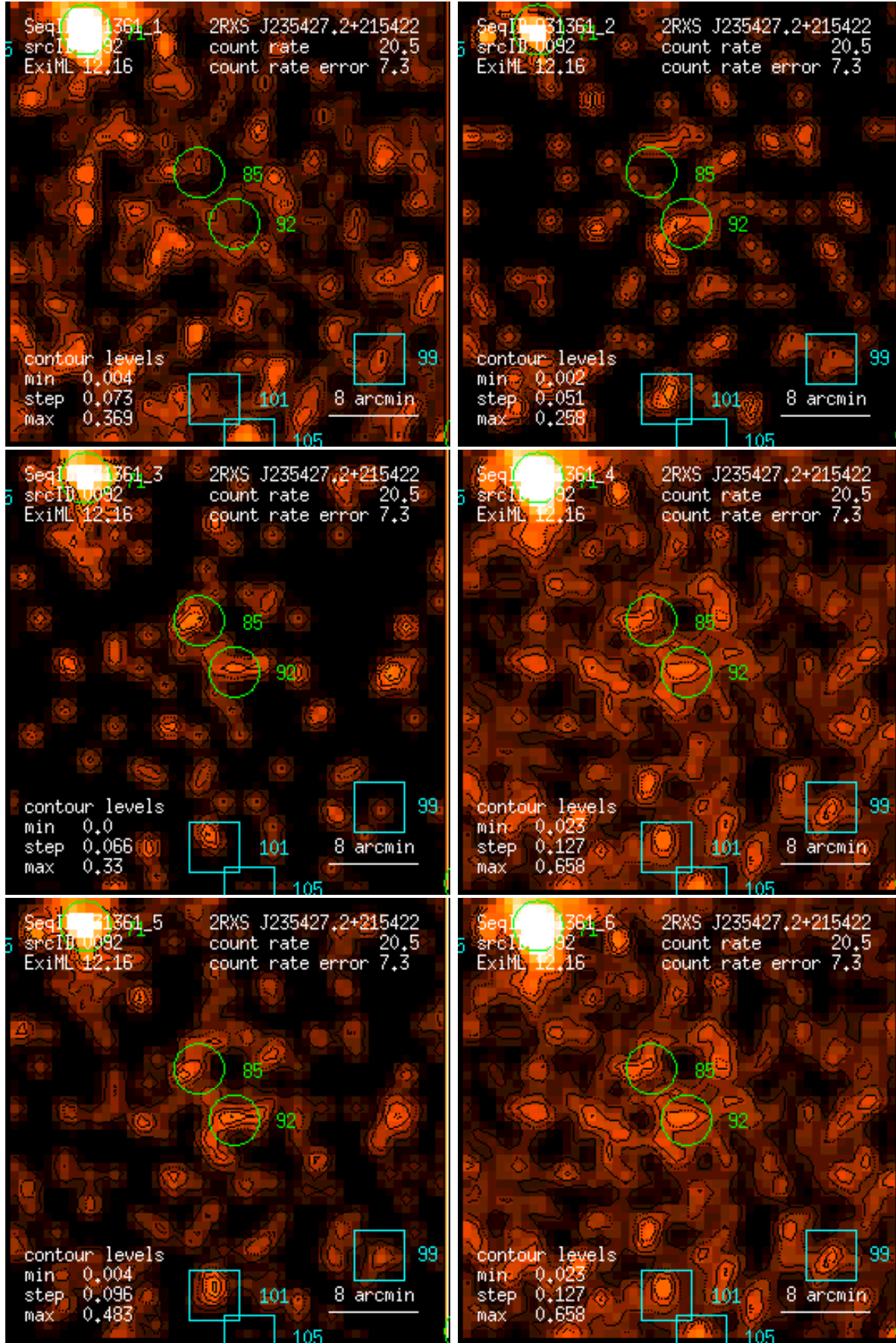
Figure 92: RASS 931361: detection 0092: band rate images, Gaussian filter: (1) PSPC channels 11 – 41, (2) 52 – 90, (3) 91 – 201, (4) 11 – 235, (5) 52 – 201, (6) 11 – 201. Broad band rates in counts/ks. Band rate contour levels in counts/ks/arcmin 2 .
