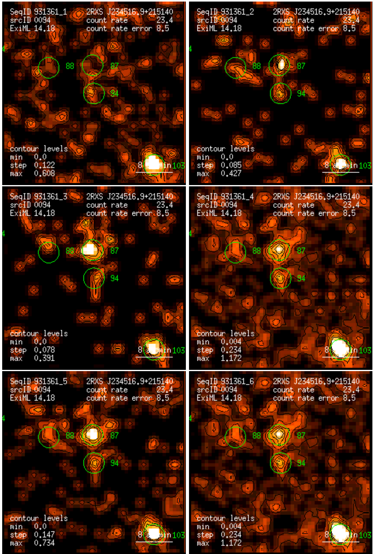
Figure 94: RASS 931361: detection 0094: band rate images, Gaussian filter: (1) PSPC channels 11 – 41, (2) 52 – 90, (3) 91 – 201, (4) 11 – 235, (5) 52 – 201, (6) 11 – 201. Broad band rates in counts/ks. Band rate contour levels in counts/ks/arcmin 2 .
