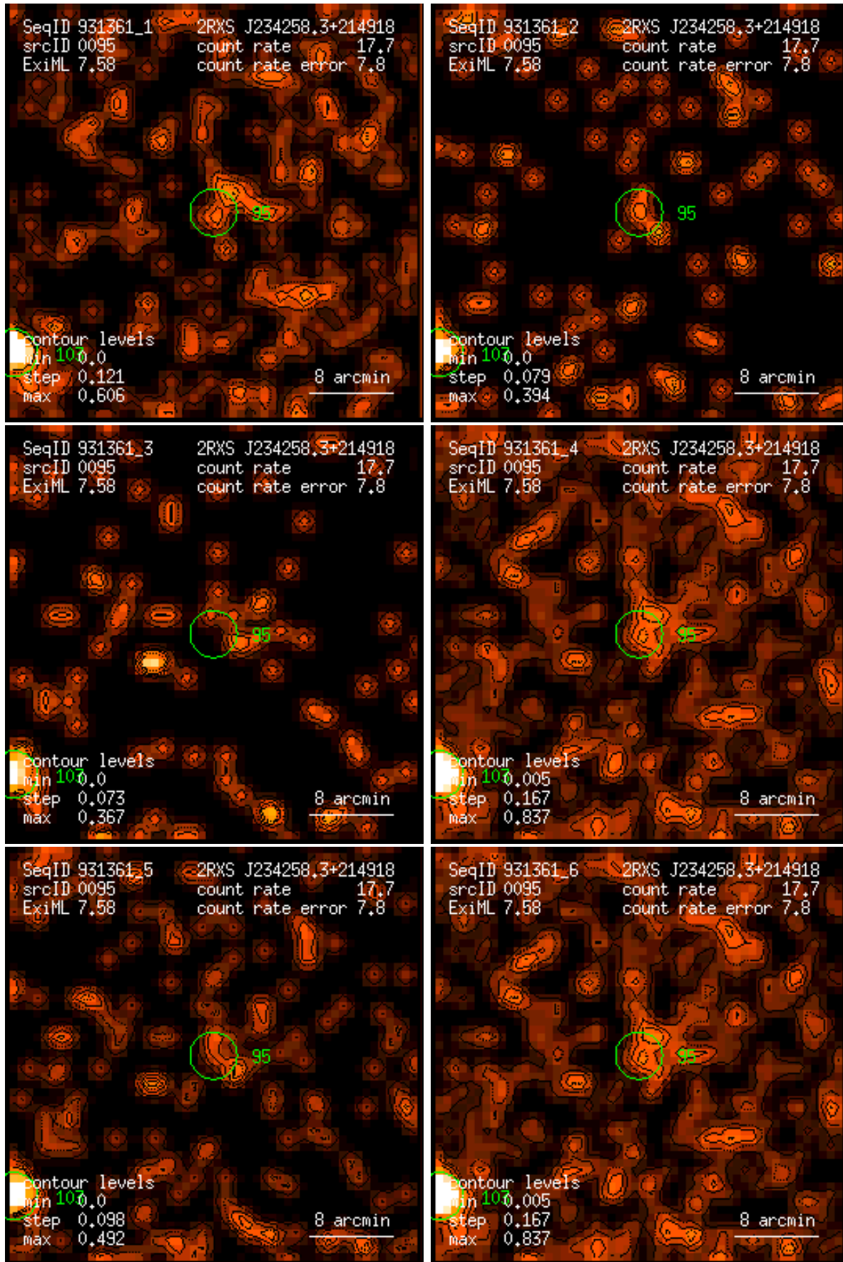
Figure 95: RASS 931361: detection 0095: band rate images, Gaussian filter: (1) PSPC channels 11 – 41, (2) 52 – 90, (3) 91 – 201, (4) 11 – 235, (5) 52 – 201, (6) 11 – 201. Broad band rates in counts/ks. Band rate contour levels in counts/ks/arcmin 2 .
