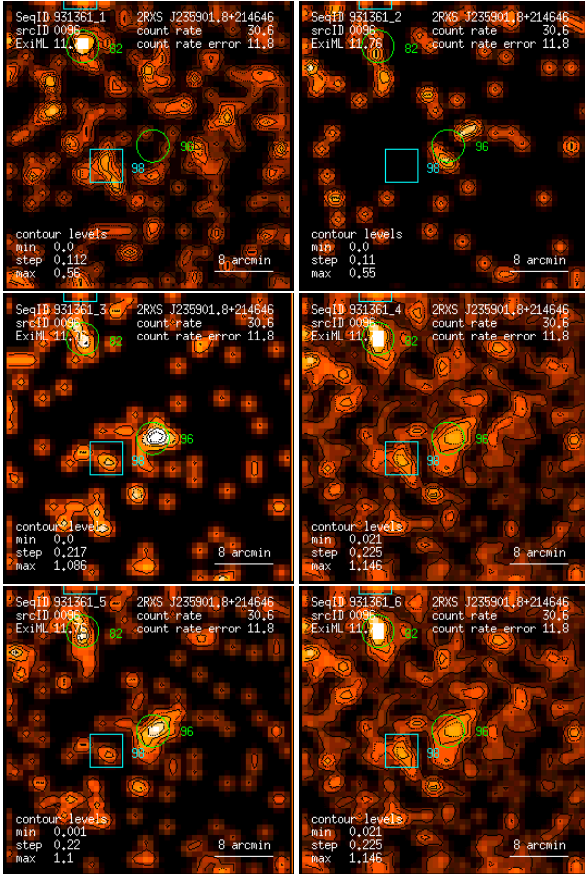
Figure 96: RASS 931361: detection 0096: band rate images, Gaussian filter: (1) PSPC channels 11 – 41, (2) 52 – 90, (3) 91 – 201, (4) 11 – 235, (5) 52 – 201, (6) 11 – 201. Broad band rates in counts/ks. Band rate contour levels in counts/ks/arcmin 2 .
