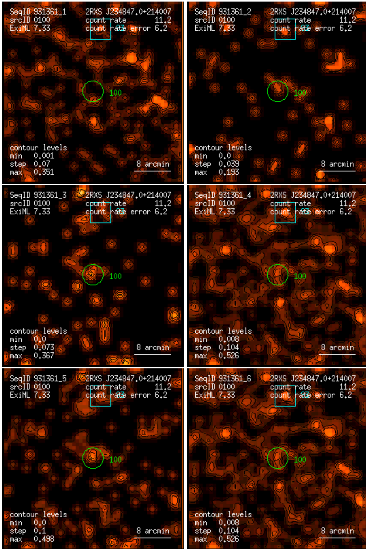
Figure 100: RASS 931361: detection 0100: band rate images, Gaussian filter: (1) PSPC channels 11 – 41, (2) 52 – 90, (3) 91 – 201, (4) 11 – 235, (5) 52 – 201, (6) 11 – 201. Broad band rates in counts/ks. Band rate contour levels in counts/ks/arcmin 2 .
