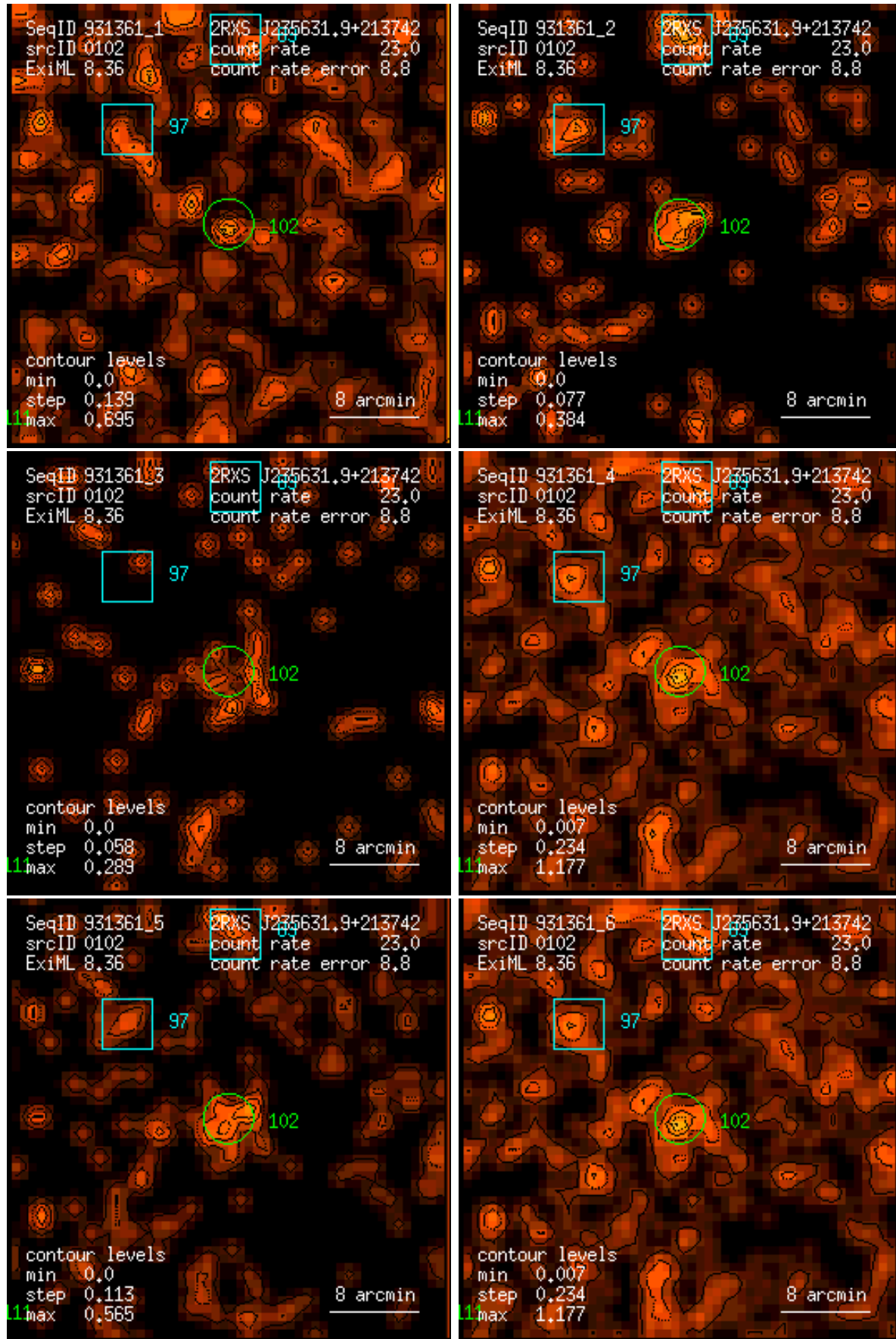
Figure 102: RASS 931361: detection 0102: band rate images, Gaussian filter: (1) PSPC channels 11 – 41, (2) 52 – 90, (3) 91 – 201, (4) 11 – 235, (5) 52 – 201, (6) 11 – 201. Broad band rates in counts/ks. Band rate contour levels in counts/ks/arcmin 2 .
