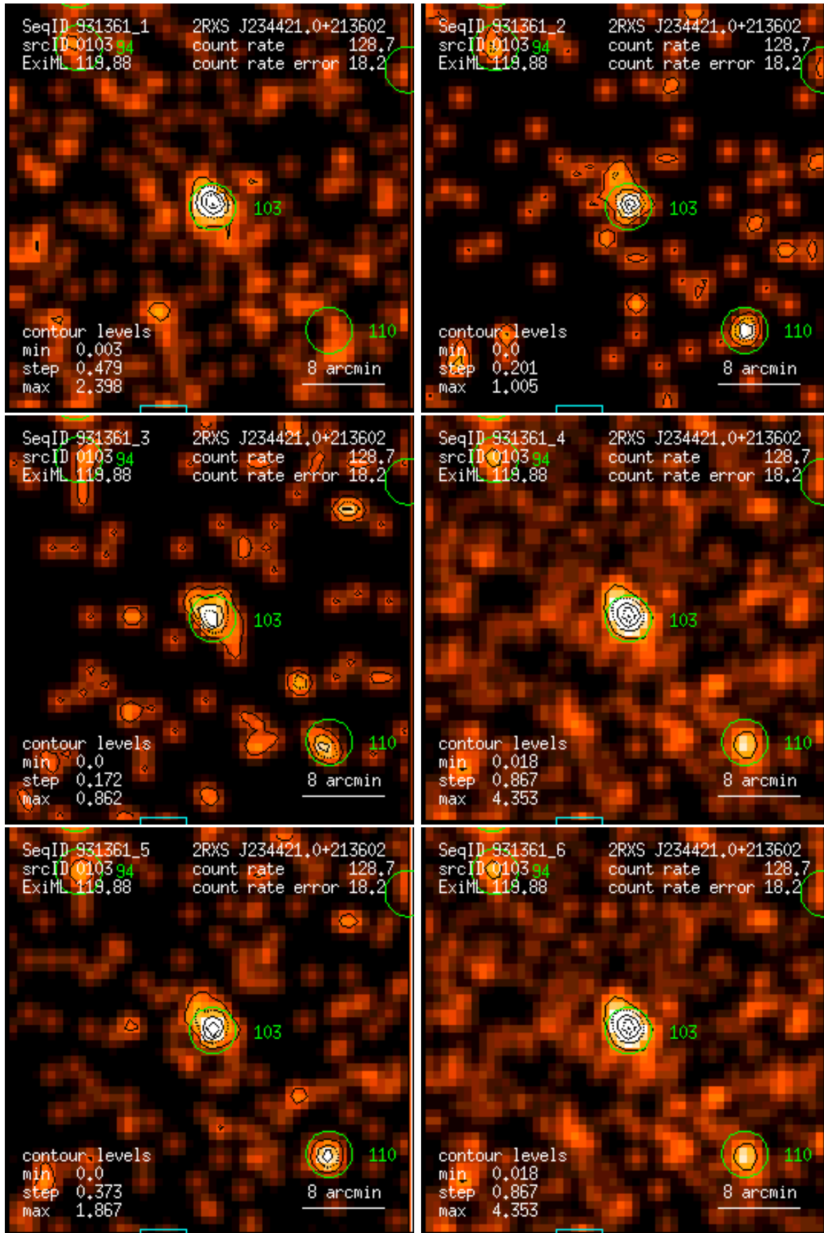
Figure 103: RASS 931361: detection 0103: band rate images, Gaussian filter: (1) PSPC channels 11 – 41, (2) 52 – 90, (3) 91 – 201, (4) 11 – 235, (5) 52 – 201, (6) 11 – 201. Broad band rates in counts/ks. Band rate contour levels in counts/ks/arcmin 2 .
