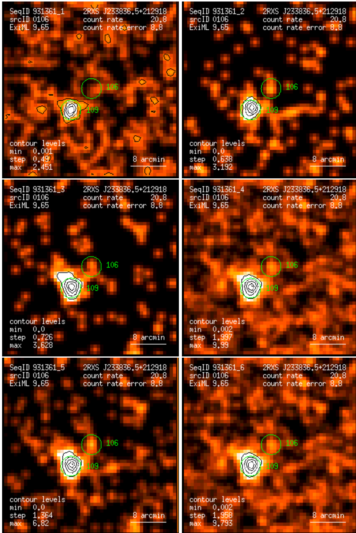
Figure 106: RASS 931361: detection 0106: band rate images, Gaussian filter: (1) PSPC channels 11 – 41, (2) 52 – 90, (3) 91 – 201, (4) 11 – 235, (5) 52 – 201, (6) 11 – 201. Broad band rates in counts/ks. Band rate contour levels in counts/ks/arcmin 2 .
